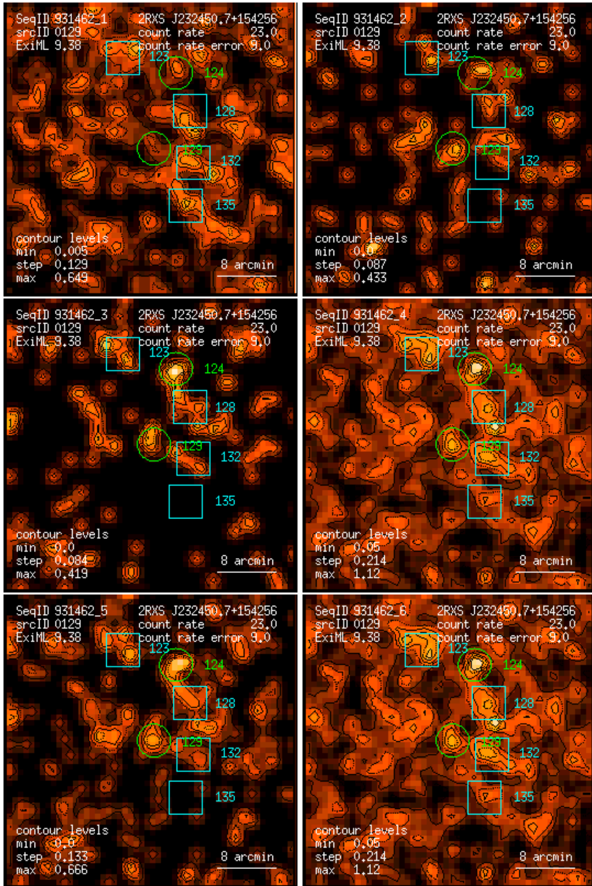
Figure 129: RASS 931462: detection 0129: band rate images, Gaussian filter: (1) PSPC channels 11 – 41, (2) 52 – 90, (3) 91 – 201, (4) 11 – 235, (5) 52 – 201, (6) 11 – 201. Broad band rates in counts/ks. Band rate contour levels in counts/ks/arcmin 2 .
