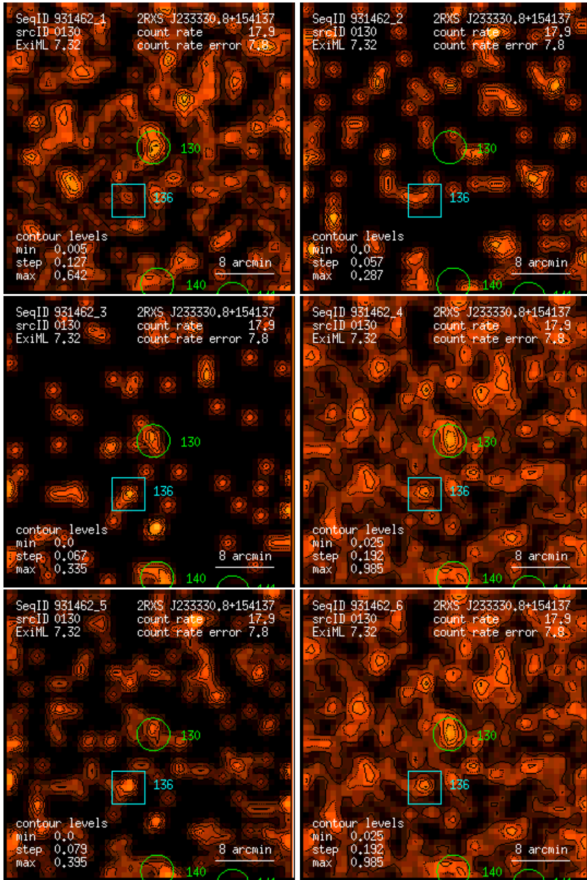
Figure 130: RASS 931462: detection 0130: band rate images, Gaussian filter: (1) PSPC channels 11 – 41, (2) 52 – 90, (3) 91 – 201, (4) 11 – 235, (5) 52 – 201, (6) 11 – 201. Broad band rates in counts/ks. Band rate contour levels in counts/ks/arcmin 2 .
