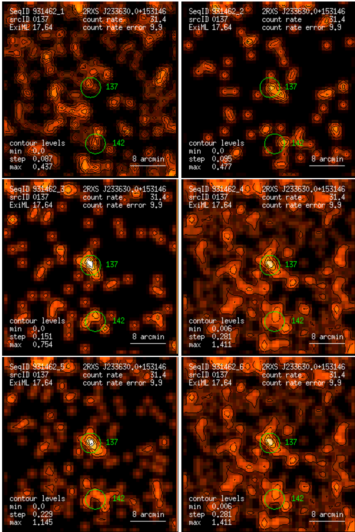
Figure 137: RASS 931462: detection 0137: band rate images, Gaussian filter: (1) PSPC channels 11 – 41, (2) 52 – 90, (3) 91 – 201, (4) 11 – 235, (5) 52 – 201, (6) 11 – 201. Broad band rates in counts/ks. Band rate contour levels in counts/ks/arcmin 2 .
