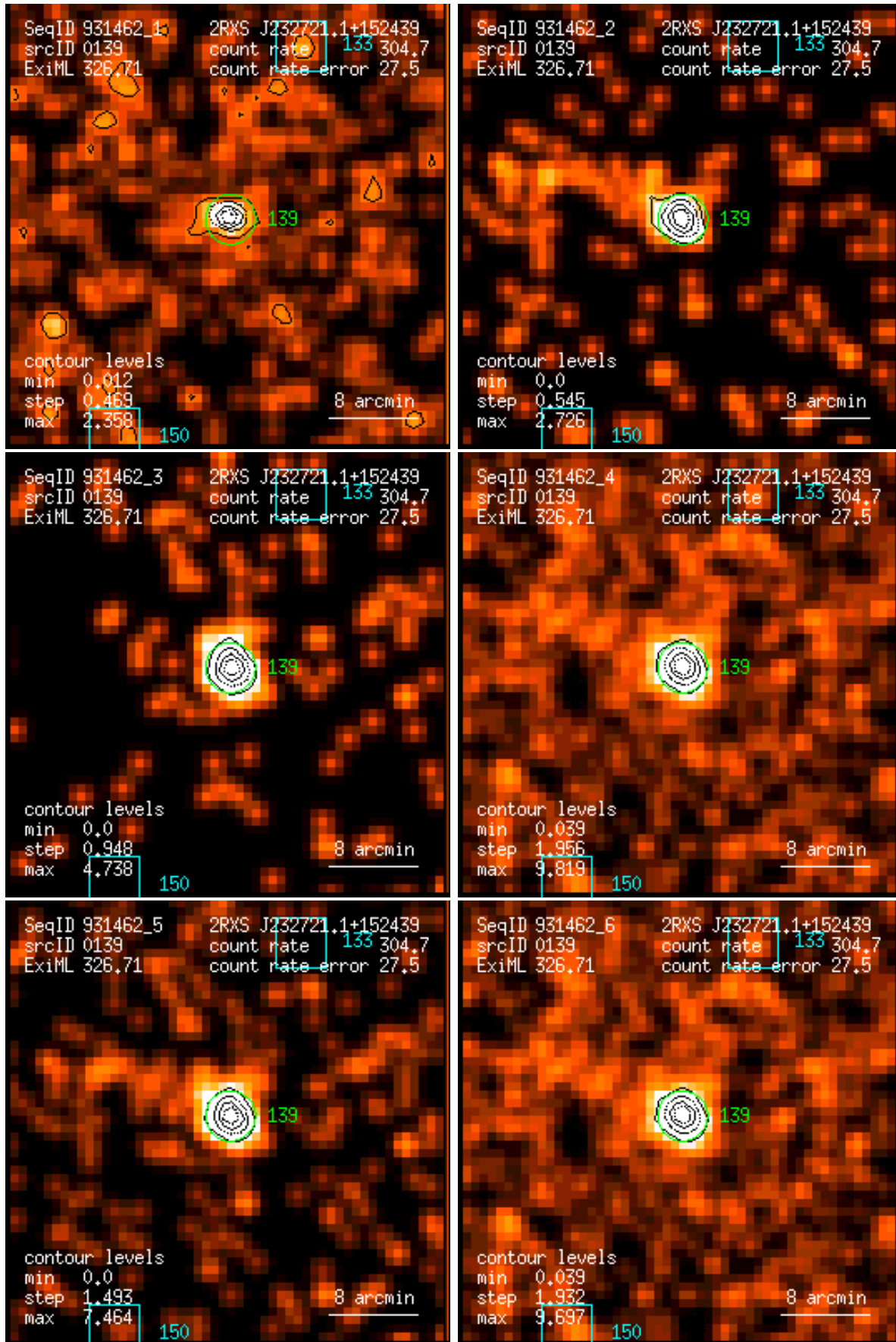
Figure 139: RASS 931462: detection 0139: band rate images, Gaussian filter: (1) PSPC channels 11 – 41, (2) 52 – 90, (3) 91 – 201, (4) 11 – 235, (5) 52 – 201, (6) 11 – 201. Broad band rates in counts/ks. Band rate contour levels in counts/ks/arcmin 2 .
