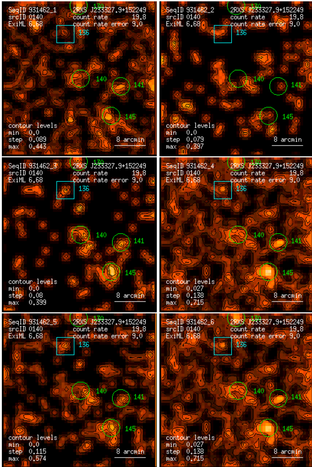
Figure 140: RASS 931462: detection 0140: band rate images, Gaussian filter: (1) PSPC channels 11 – 41, (2) 52 – 90, (3) 91 – 201, (4) 11 – 235, (5) 52 – 201, (6) 11 – 201. Broad band rates in counts/ks. Band rate contour levels in counts/ks/arcmin 2 .
