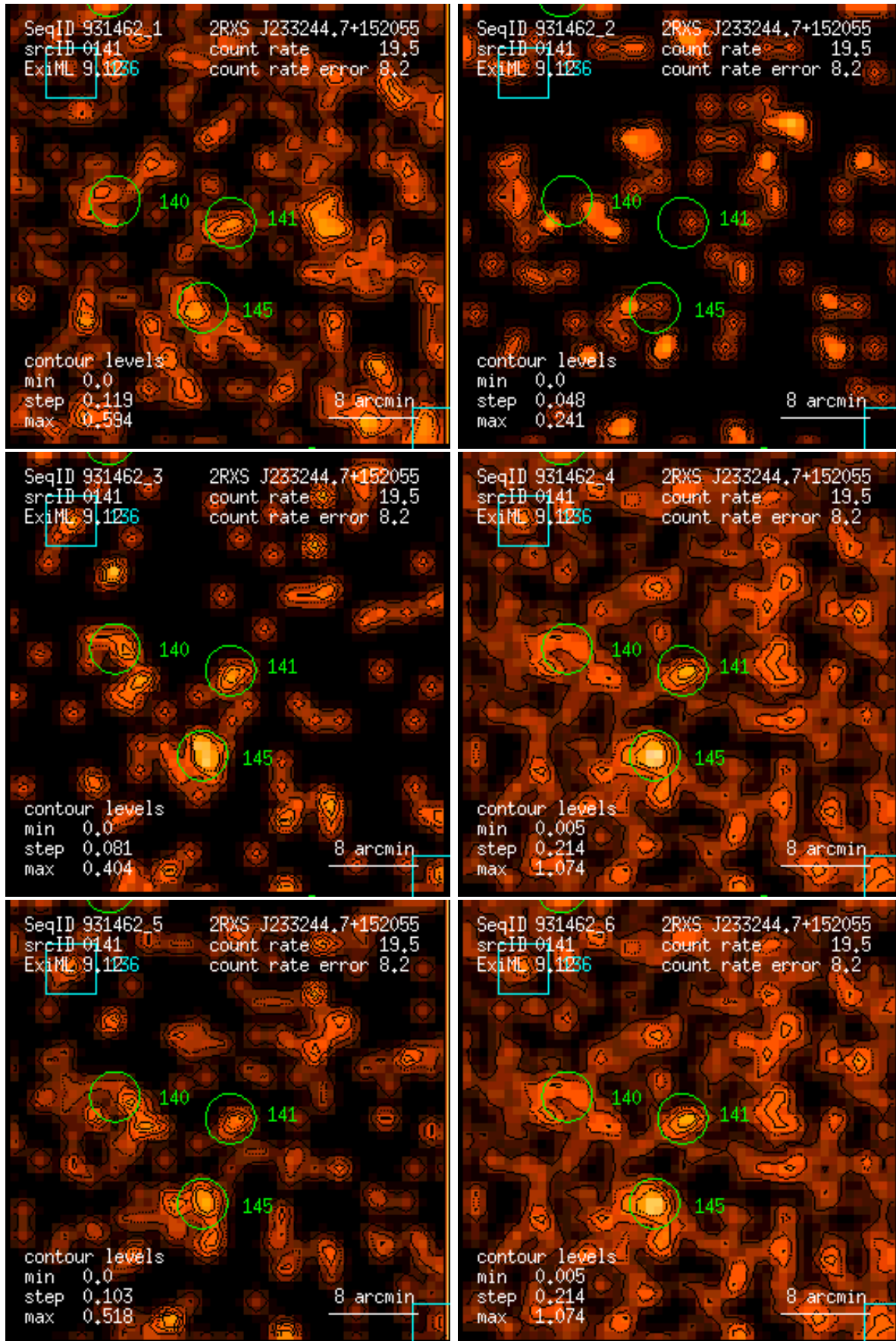
Figure 141: RASS 931462: detection 0141: band rate images, Gaussian filter: (1) PSPC channels 11 – 41, (2) 52 – 90, (3) 91 – 201, (4) 11 – 235, (5) 52 – 201, (6) 11 – 201. Broad band rates in counts/ks. Band rate contour levels in counts/ks/arcmin 2 .
