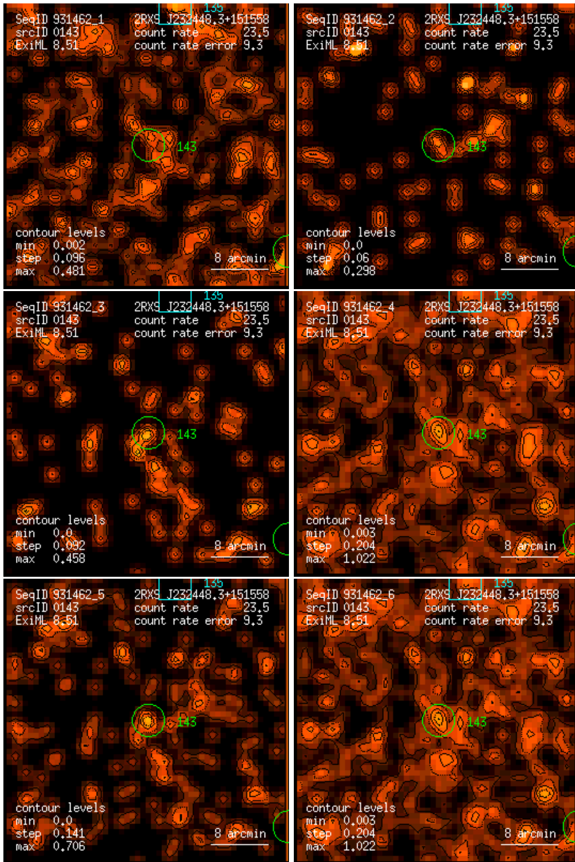
Figure 143: RASS 931462: detection 0143: band rate images, Gaussian filter: (1) PSPC channels 11 – 41, (2) 52 – 90, (3) 91 – 201, (4) 11 – 235, (5) 52 – 201, (6) 11 – 201. Broad band rates in counts/ks. Band rate contour levels in counts/ks/arcmin 2 .
