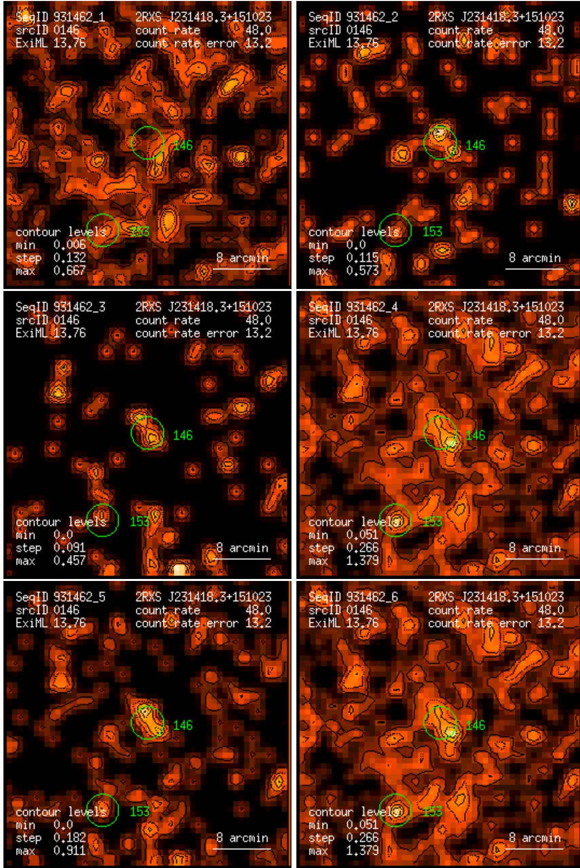
Figure 146: RASS 931462: detection 0146: band rate images, Gaussian filter: (1) PSPC channels 11 – 41, (2) 52 – 90, (3) 91 – 201, (4) 11 – 235, (5) 52 – 201, (6) 11 – 201. Broad band rates in counts/ks. Band rate contour levels in counts/ks/arcmin 2 .
