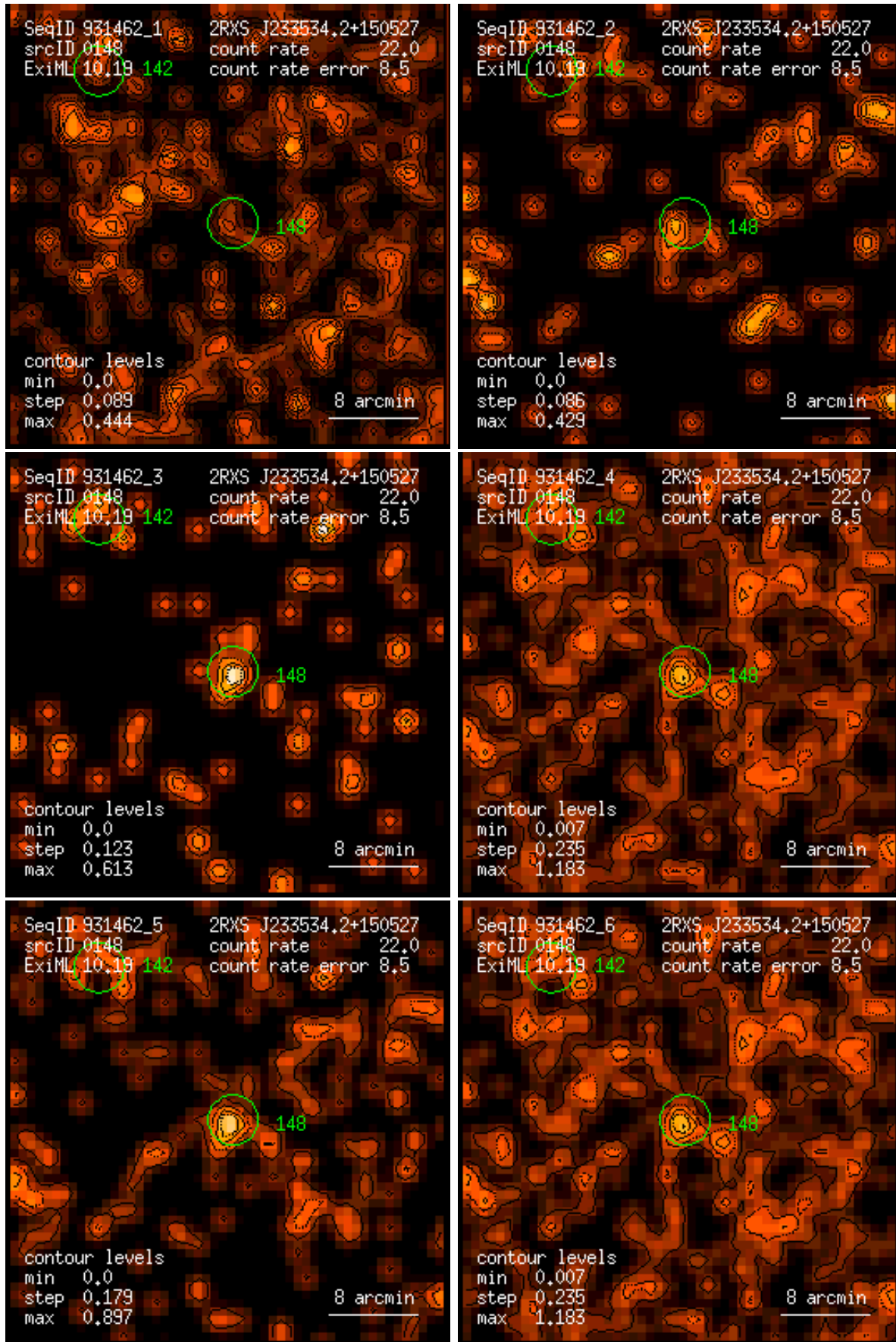
Figure 148: RASS 931462: detection 0148: band rate images, Gaussian filter: (1) PSPC channels 11 – 41, (2) 52 – 90, (3) 91 – 201, (4) 11 – 235, (5) 52 – 201, (6) 11 – 201. Broad band rates in counts/ks. Band rate contour levels in counts/ks/arcmin 2 .
