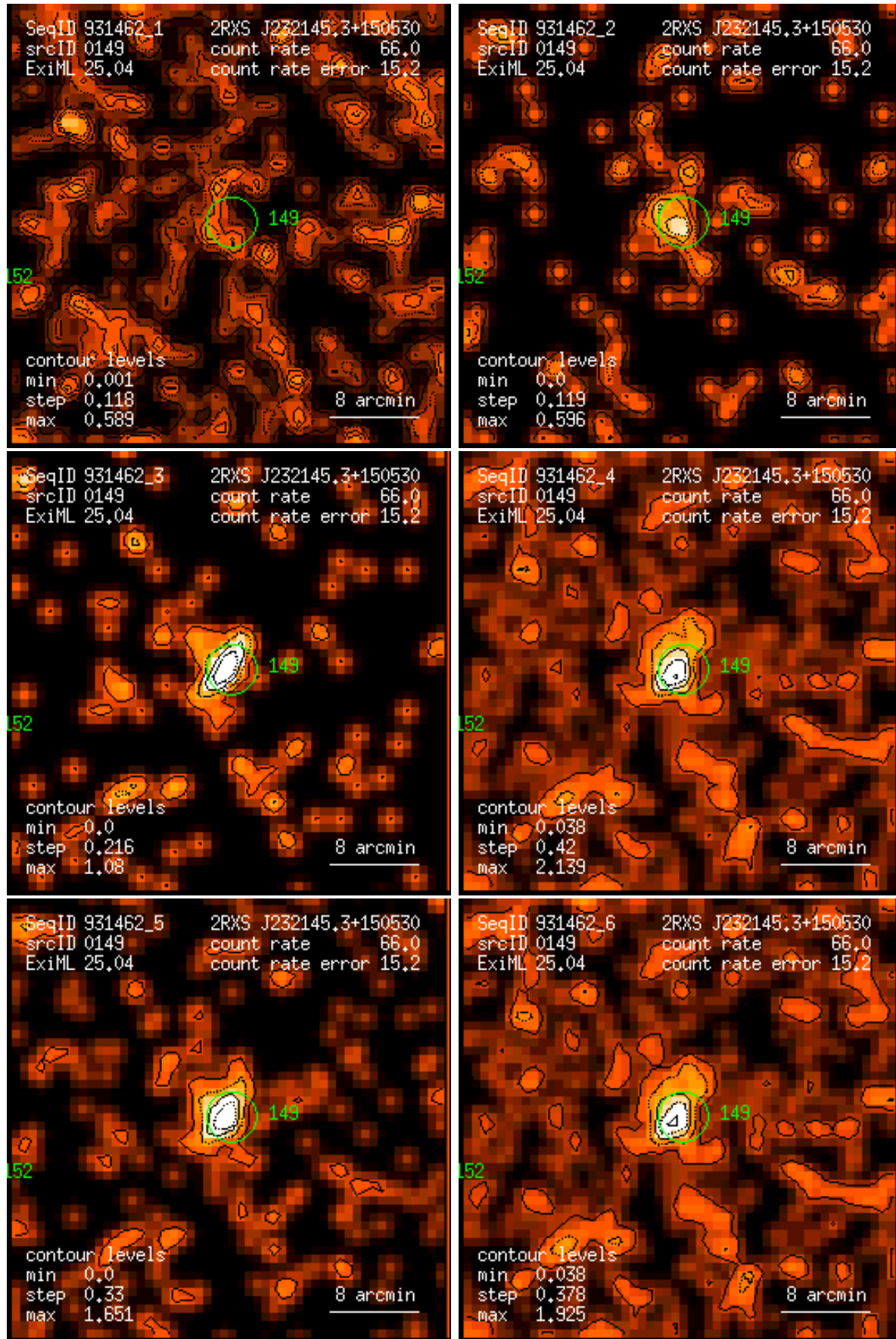
Figure 149: RASS 931462: detection 0149: band rate images, Gaussian filter: (1) PSPC channels 11 – 41, (2) 52 – 90, (3) 91 – 201, (4) 11 – 235, (5) 52 – 201, (6) 11 – 201. Broad band rates in counts/ks. Band rate contour levels in counts/ks/arcmin 2 .
