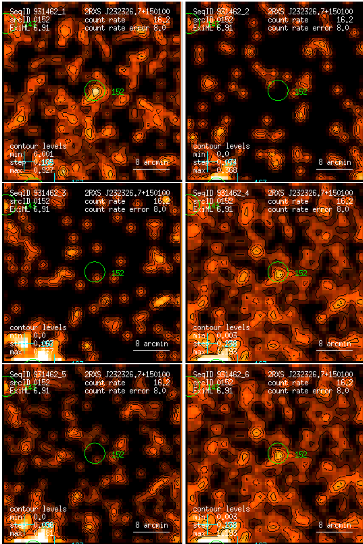
Figure 152: RASS 931462: detection 0152: band rate images, Gaussian filter: (1) PSPC channels 11 – 41, (2) 52 – 90, (3) 91 – 201, (4) 11 – 235, (5) 52 – 201, (6) 11 – 201. Broad band rates in counts/ks. Band rate contour levels in counts/ks/arcmin 2 .
