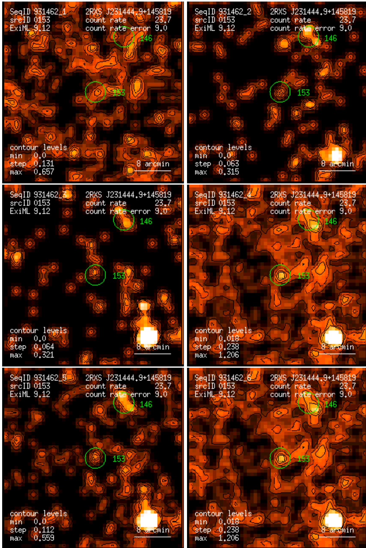
Figure 153: RASS 931462: detection 0153: band rate images, Gaussian filter: (1) PSPC channels 11 – 41, (2) 52 – 90, (3) 91 – 201, (4) 11 – 235, (5) 52 – 201, (6) 11 – 201. Broad band rates in counts/ks. Band rate contour levels in counts/ks/arcmin 2 .
