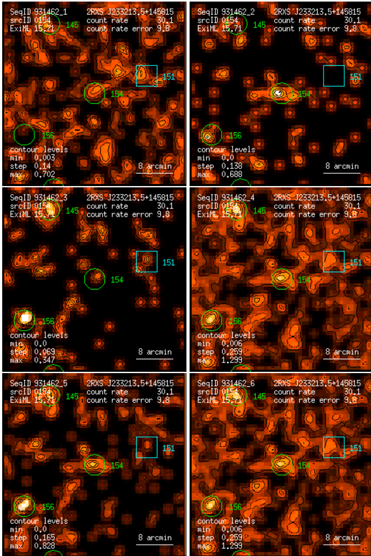
Figure 154: RASS 931462: detection 0154: band rate images, Gaussian filter: (1) PSPC channels 11 – 41, (2) 52 – 90, (3) 91 – 201, (4) 11 – 235, (5) 52 – 201, (6) 11 – 201. Broad band rates in counts/ks. Band rate contour levels in counts/ks/arcmin 2 .
