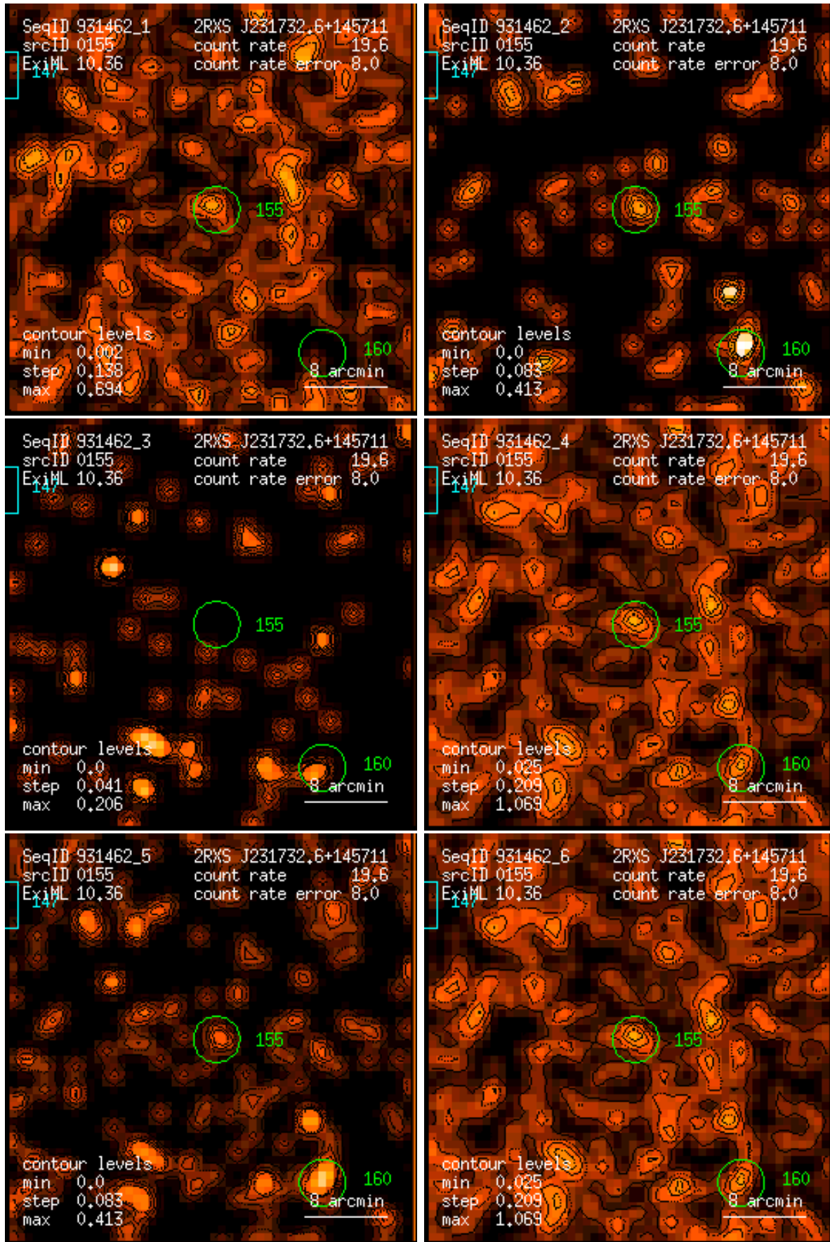
Figure 155: RASS 931462: detection 0155: band rate images, Gaussian filter: (1) PSPC channels 11 – 41, (2) 52 – 90, (3) 91 – 201, (4) 11 – 235, (5) 52 – 201, (6) 11 – 201. Broad band rates in counts/ks. Band rate contour levels in counts/ks/arcmin 2 .
