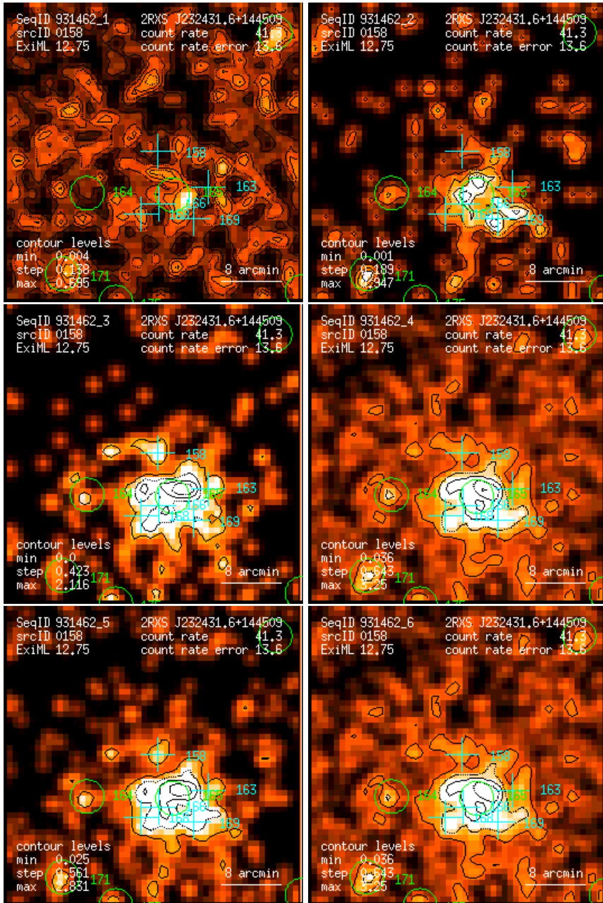
Figure 158: RASS 931462: detection 0158: band rate images, Gaussian filter: (1) PSPC channels 11 – 41, (2) 52 – 90, (3) 91 – 201, (4) 11 – 235, (5) 52 – 201, (6) 11 – 201. Broad band rates in counts/ks. Band rate contour levels in counts/ks/arcmin 2 .
