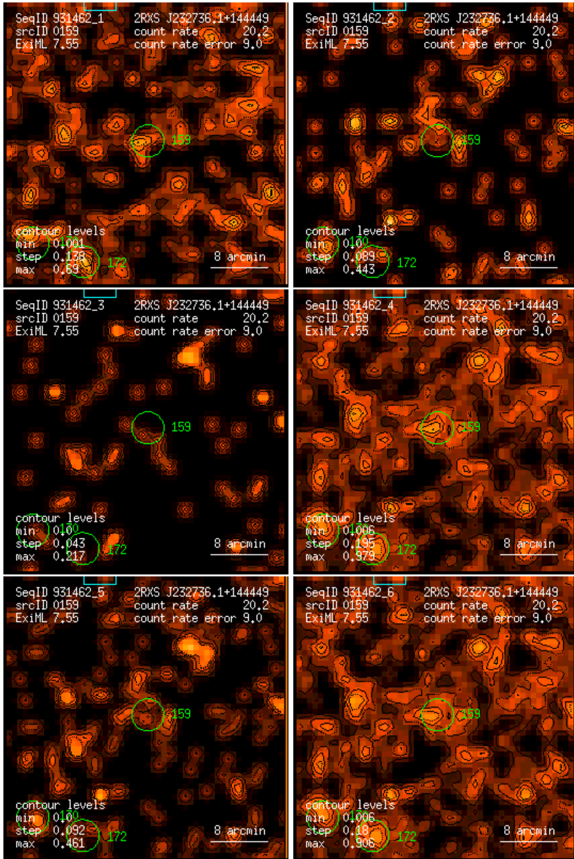
Figure 159: RASS 931462: detection 0159: band rate images, Gaussian filter: (1) PSPC channels 11 – 41, (2) 52 – 90, (3) 91 – 201, (4) 11 – 235, (5) 52 – 201, (6) 11 – 201. Broad band rates in counts/ks. Band rate contour levels in counts/ks/arcmin 2 .
