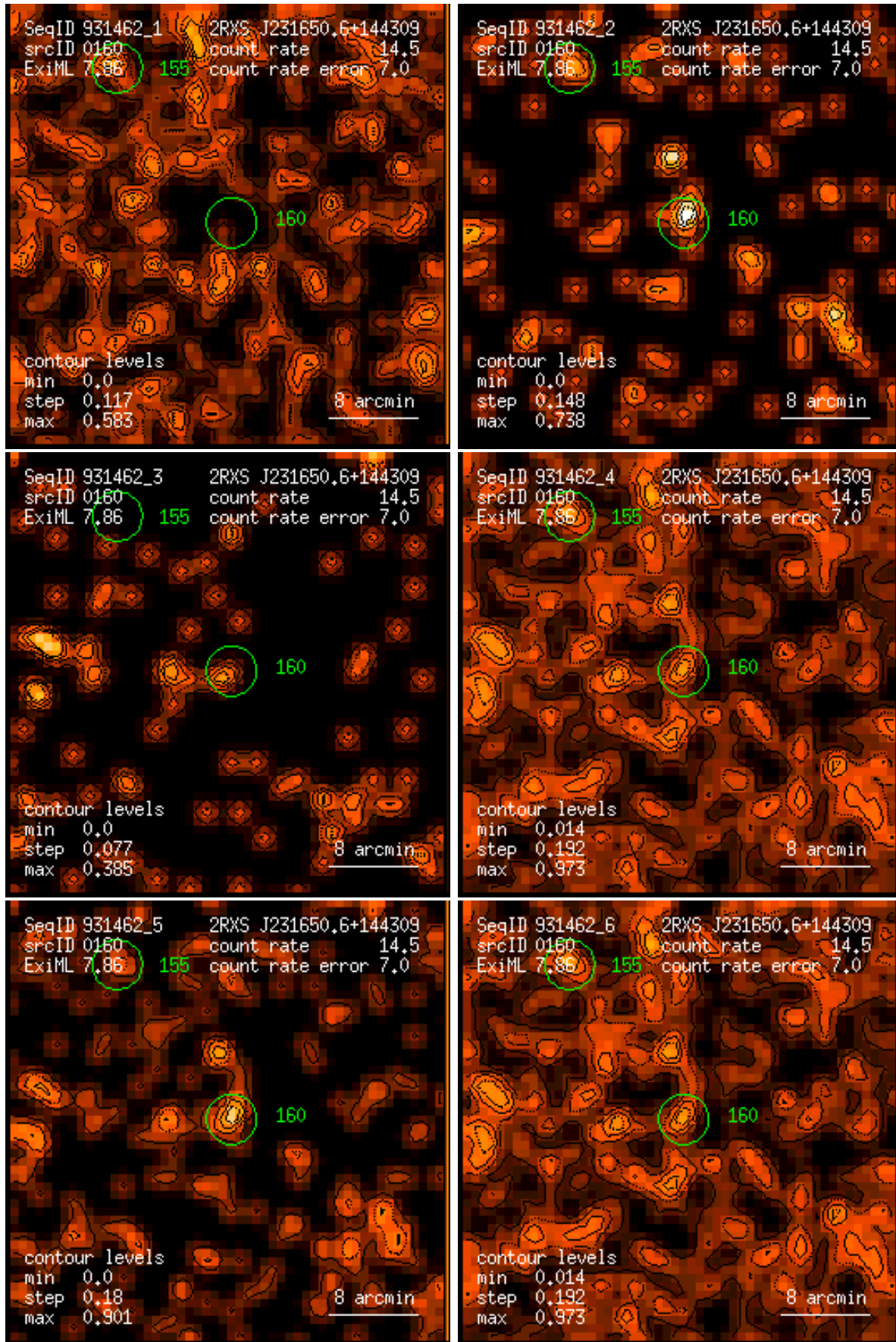
Figure 160: RASS 931462: detection 0160: band rate images, Gaussian filter: (1) PSPC channels 11 – 41, (2) 52 – 90, (3) 91 – 201, (4) 11 – 235, (5) 52 – 201, (6) 11 – 201. Broad band rates in counts/ks. Band rate contour levels in counts/ks/arcmin 2 .
