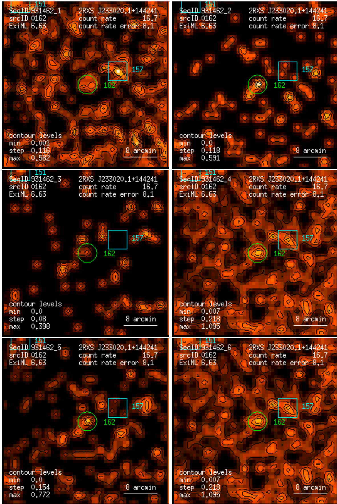
Figure 162: RASS 931462: detection 0162: band rate images, Gaussian filter: (1) PSPC channels 11 – 41, (2) 52 – 90, (3) 91 – 201, (4) 11 – 235, (5) 52 – 201, (6) 11 – 201. Broad band rates in counts/ks. Band rate contour levels in counts/ks/arcmin 2 .
