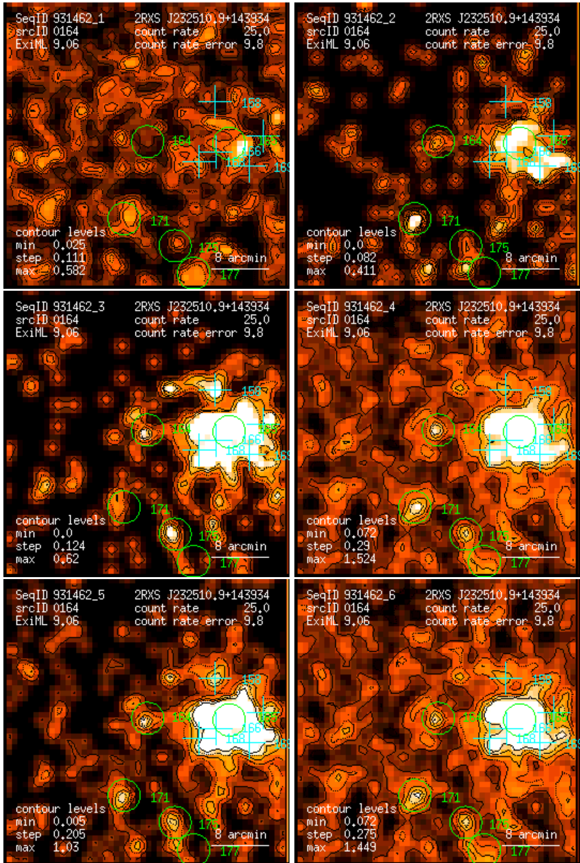
Figure 164: RASS 931462: detection 0164: band rate images, Gaussian filter: (1) PSPC channels 11 – 41, (2) 52 – 90, (3) 91 – 201, (4) 11 – 235, (5) 52 – 201, (6) 11 – 201. Broad band rates in counts/ks. Band rate contour levels in counts/ks/arcmin 2 .
