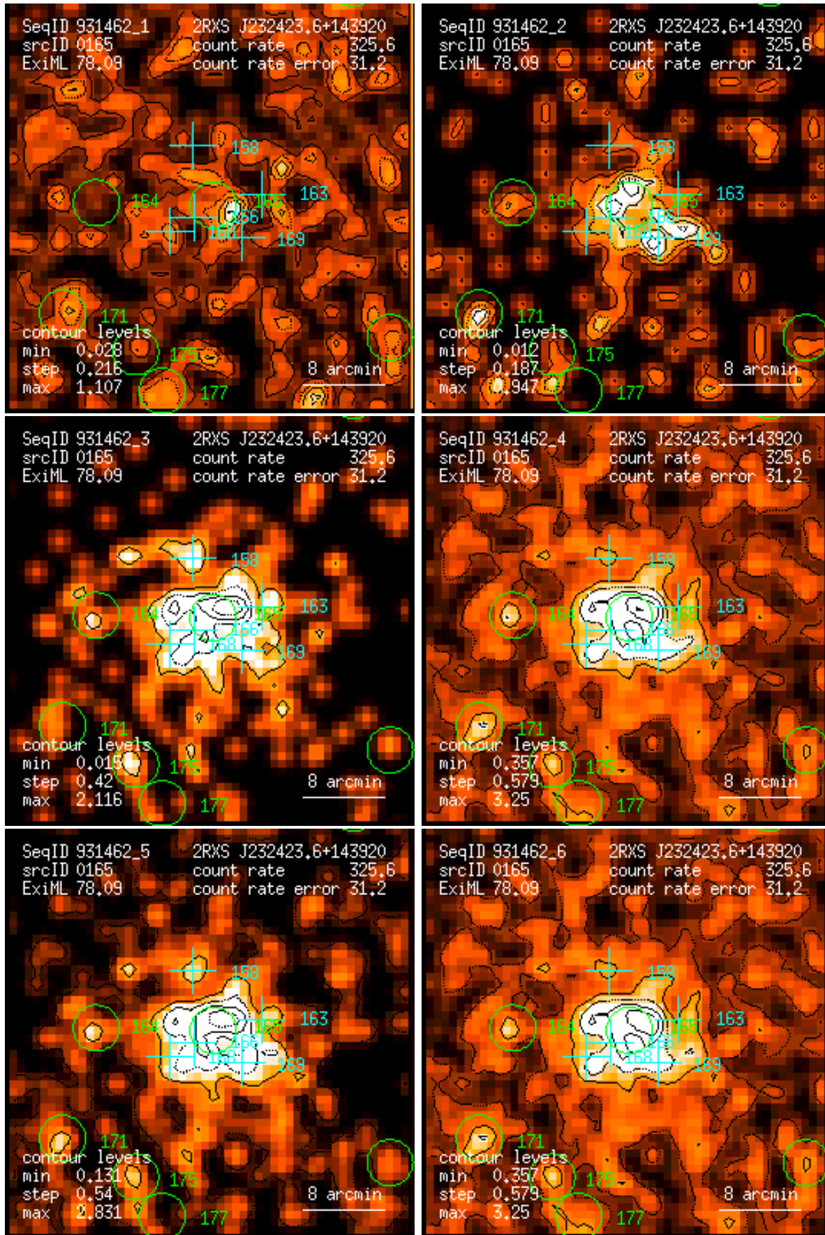
Figure 165: RASS 931462: detection 0165: band rate images, Gaussian filter: (1) PSPC channels 11 – 41, (2) 52 – 90, (3) 91 – 201, (4) 11 – 235, (5) 52 – 201, (6) 11 – 201. Broad band rates in counts/ks. Band rate contour levels in counts/ks/arcmin 2 .
