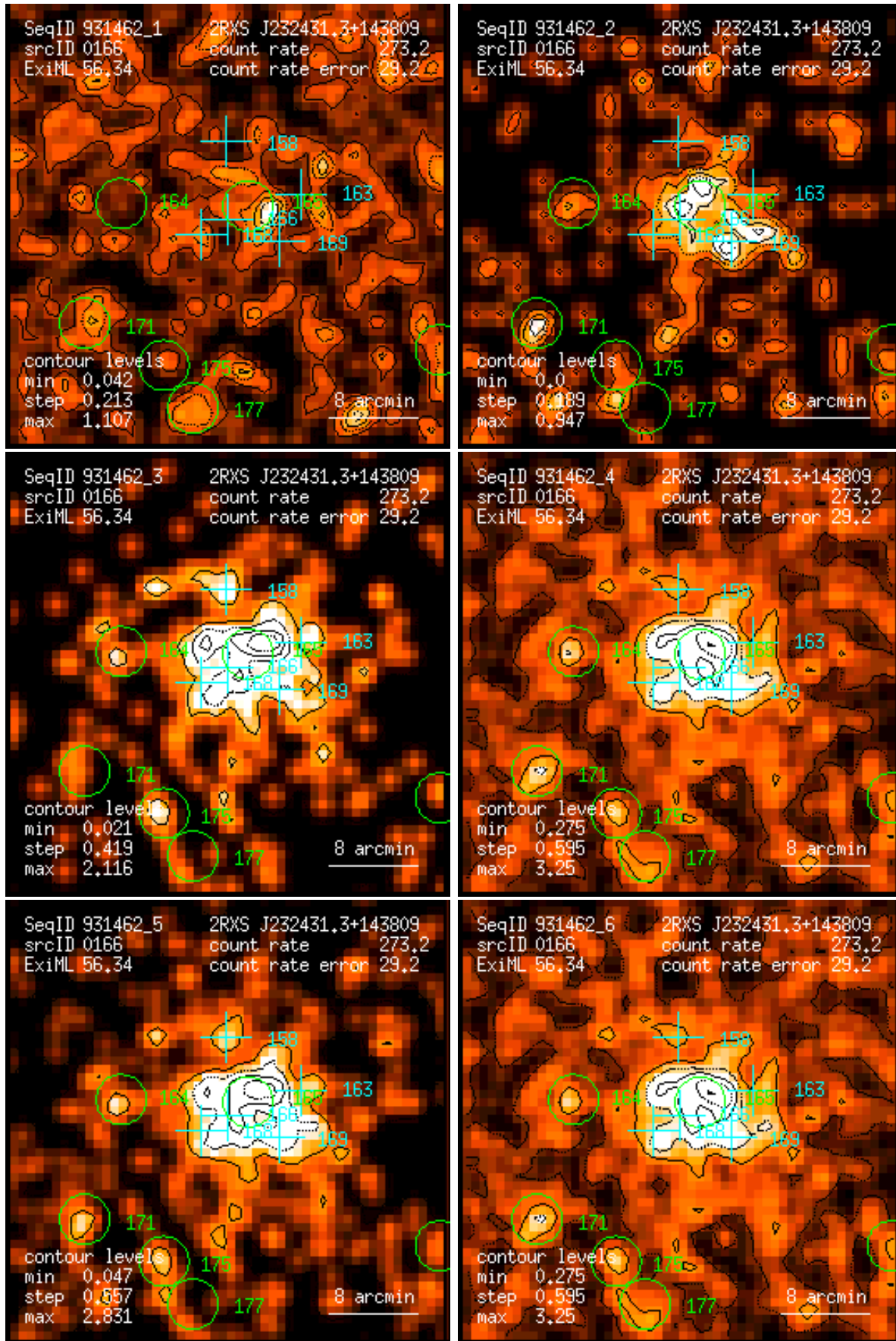
Figure 166: RASS 931462: detection 0166: band rate images, Gaussian filter: (1) PSPC channels 11 – 41, (2) 52 – 90, (3) 91 – 201, (4) 11 – 235, (5) 52 – 201, (6) 11 – 201. Broad band rates in counts/ks. Band rate contour levels in counts/ks/arcmin 2 .
