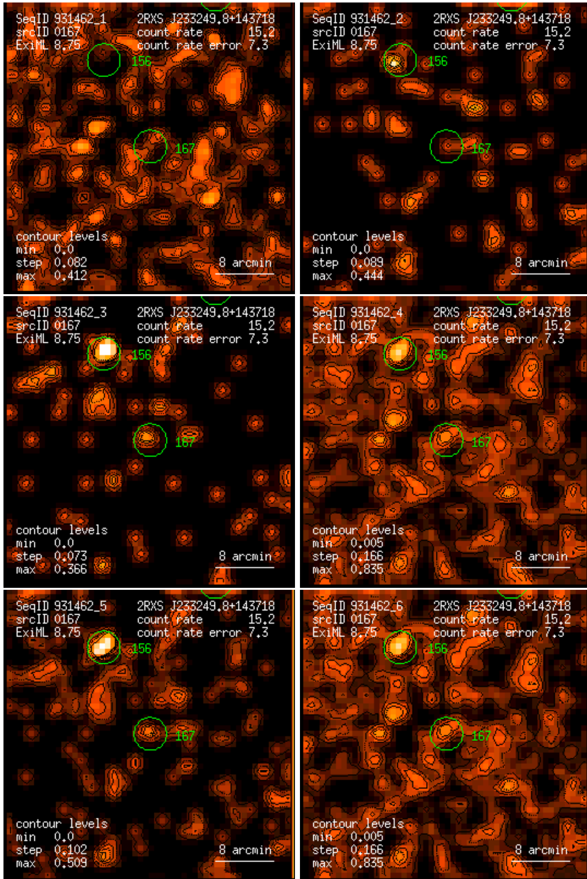
Figure 167: RASS 931462: detection 0167: band rate images, Gaussian filter: (1) PSPC channels 11 – 41, (2) 52 – 90, (3) 91 – 201, (4) 11 – 235, (5) 52 – 201, (6) 11 – 201. Broad band rates in counts/ks. Band rate contour levels in counts/ks/arcmin 2 .
