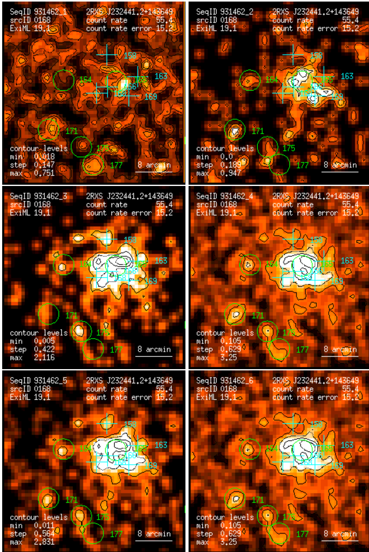
Figure 168: RASS 931462: detection 0168: band rate images, Gaussian filter: (1) PSPC channels 11 – 41, (2) 52 – 90, (3) 91 – 201, (4) 11 – 235, (5) 52 – 201, (6) 11 – 201. Broad band rates in counts/ks. Band rate contour levels in counts/ks/arcmin 2 .
