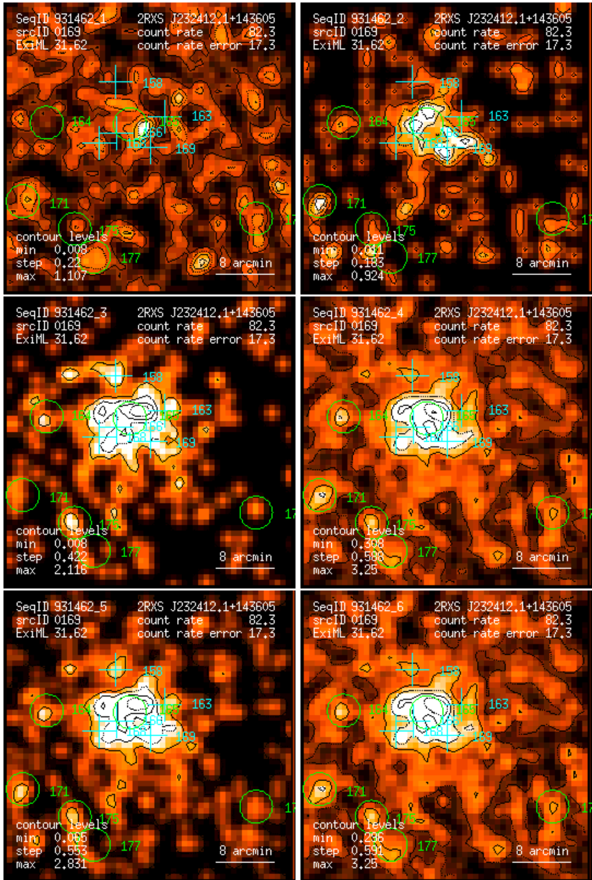
Figure 169: RASS 931462: detection 0169: band rate images, Gaussian filter: (1) PSPC channels 11 – 41, (2) 52 – 90, (3) 91 – 201, (4) 11 – 235, (5) 52 – 201, (6) 11 – 201. Broad band rates in counts/ks. Band rate contour levels in counts/ks/arcmin 2 .
