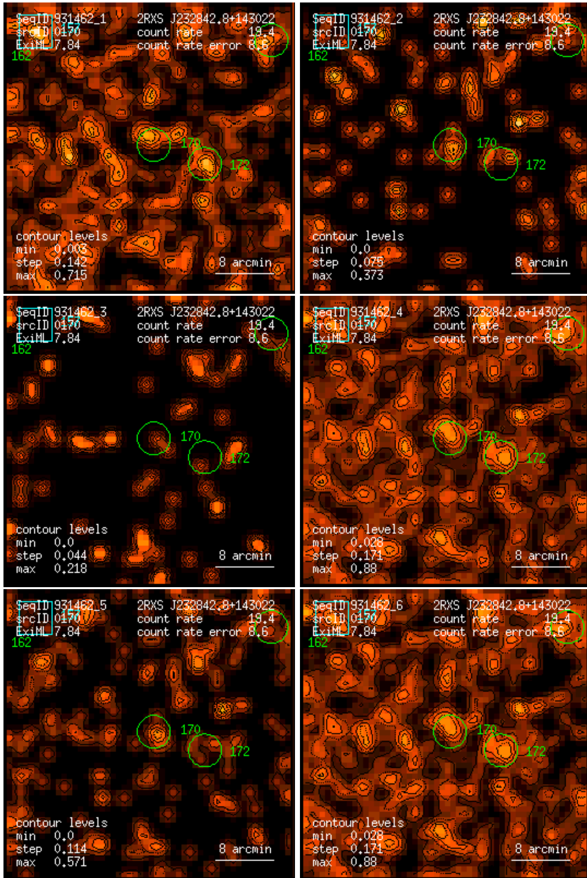
Figure 170: RASS 931462: detection 0170: band rate images, Gaussian filter: (1) PSPC channels 11 – 41, (2) 52 – 90, (3) 91 – 201, (4) 11 – 235, (5) 52 – 201, (6) 11 – 201. Broad band rates in counts/ks. Band rate contour levels in counts/ks/arcmin 2 .
