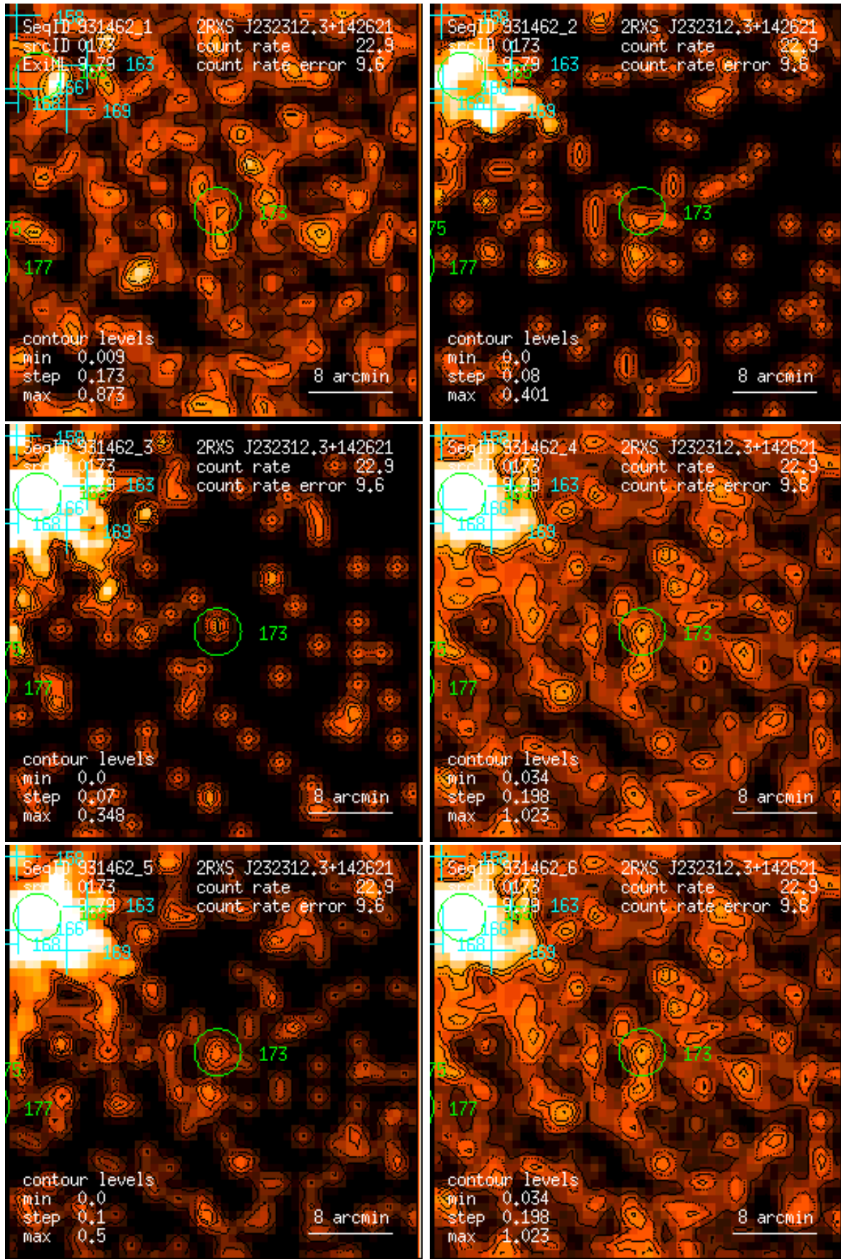
Figure 173: RASS 931462: detection 0173: band rate images, Gaussian filter: (1) PSPC channels 11 – 41, (2) 52 – 90, (3) 91 – 201, (4) 11 – 235, (5) 52 – 201, (6) 11 – 201. Broad band rates in counts/ks. Band rate contour levels in counts/ks/arcmin 2 .
