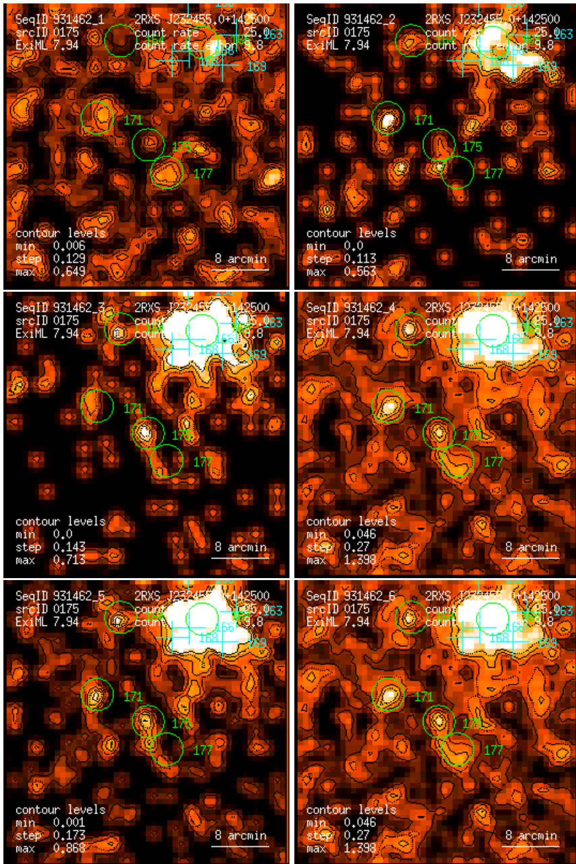
Figure 175: RASS 931462: detection 0175: band rate images, Gaussian filter: (1) PSPC channels 11 – 41, (2) 52 – 90, (3) 91 – 201, (4) 11 – 235, (5) 52 – 201, (6) 11 – 201. Broad band rates in counts/ks. Band rate contour levels in counts/ks/arcmin 2 .
