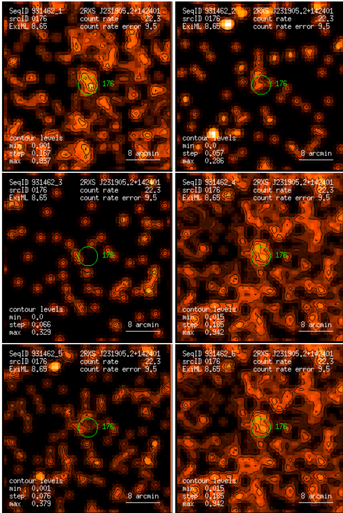
Figure 176: RASS 931462: detection 0176: band rate images, Gaussian filter: (1) PSPC channels 11 – 41, (2) 52 – 90, (3) 91 – 201, (4) 11 – 235, (5) 52 – 201, (6) 11 – 201. Broad band rates in counts/ks. Band rate contour levels in counts/ks/arcmin 2 .
