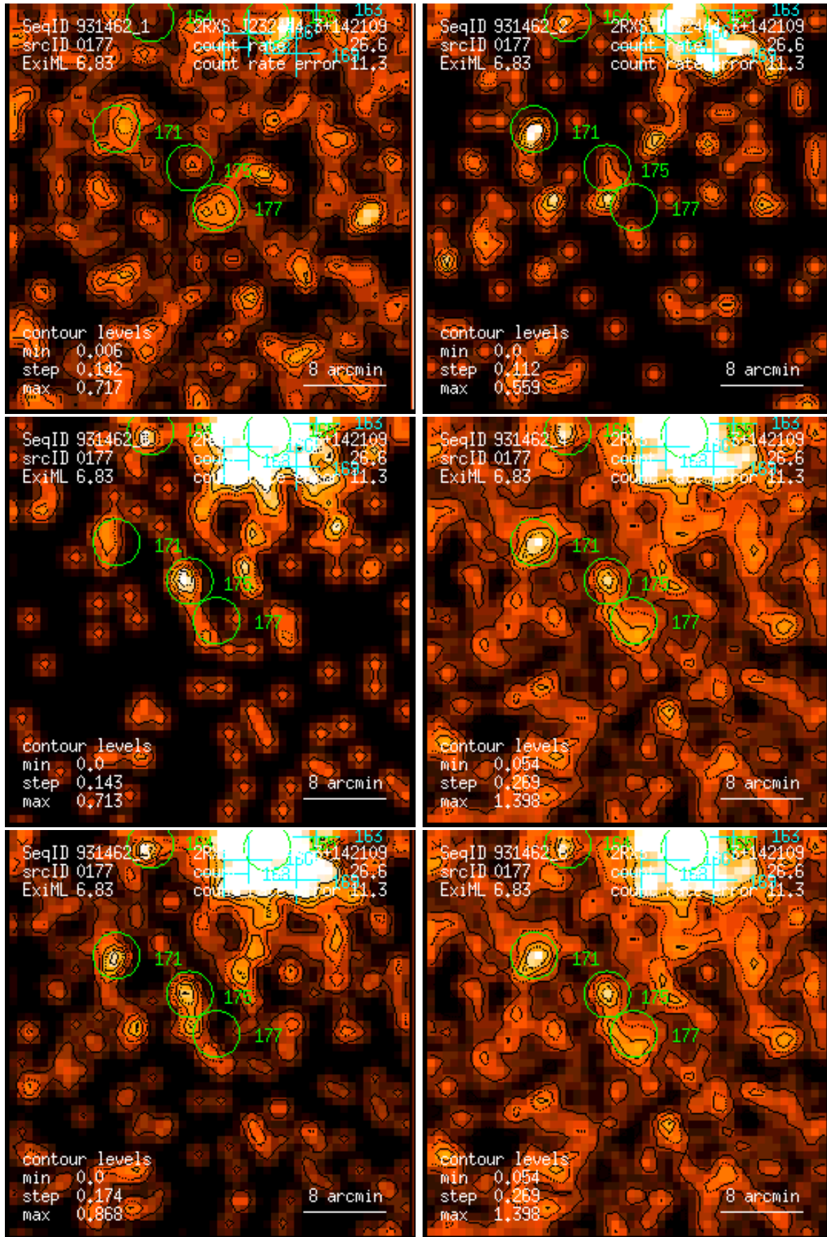
Figure 177: RASS 931462: detection 0177: band rate images, Gaussian filter: (1) PSPC channels 11 – 41, (2) 52 – 90, (3) 91 – 201, (4) 11 – 235, (5) 52 – 201, (6) 11 – 201. Broad band rates in counts/ks. Band rate contour levels in counts/ks/arcmin 2 .
