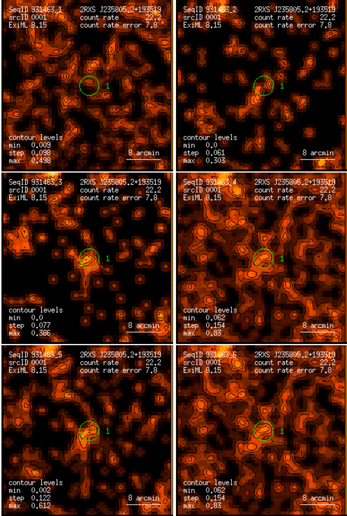
Figure 1: RASS 931463: detection 0001: band rate images, Gaussian filter: (1) PSPC channels 11 – 41, (2) 52 – 90, (3) 91 – 201, (4) 11 – 235, (5) 52 – 201, (6) 11 – 201. Broad band rates in counts/ks. Band rate contour levels in counts/ks/arcmin 2 .
