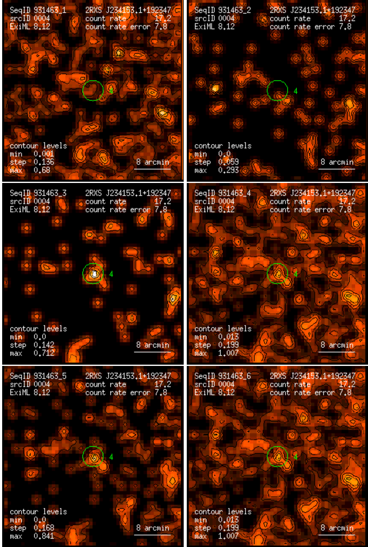
Figure 4: RASS 931463: detection 0004: band rate images, Gaussian filter: (1) PSPC channels 11 – 41, (2) 52 – 90, (3) 91 – 201, (4) 11 – 235, (5) 52 – 201, (6) 11 – 201. Broad band rates in counts/ks. Band rate contour levels in counts/ks/arcmin 2 .
