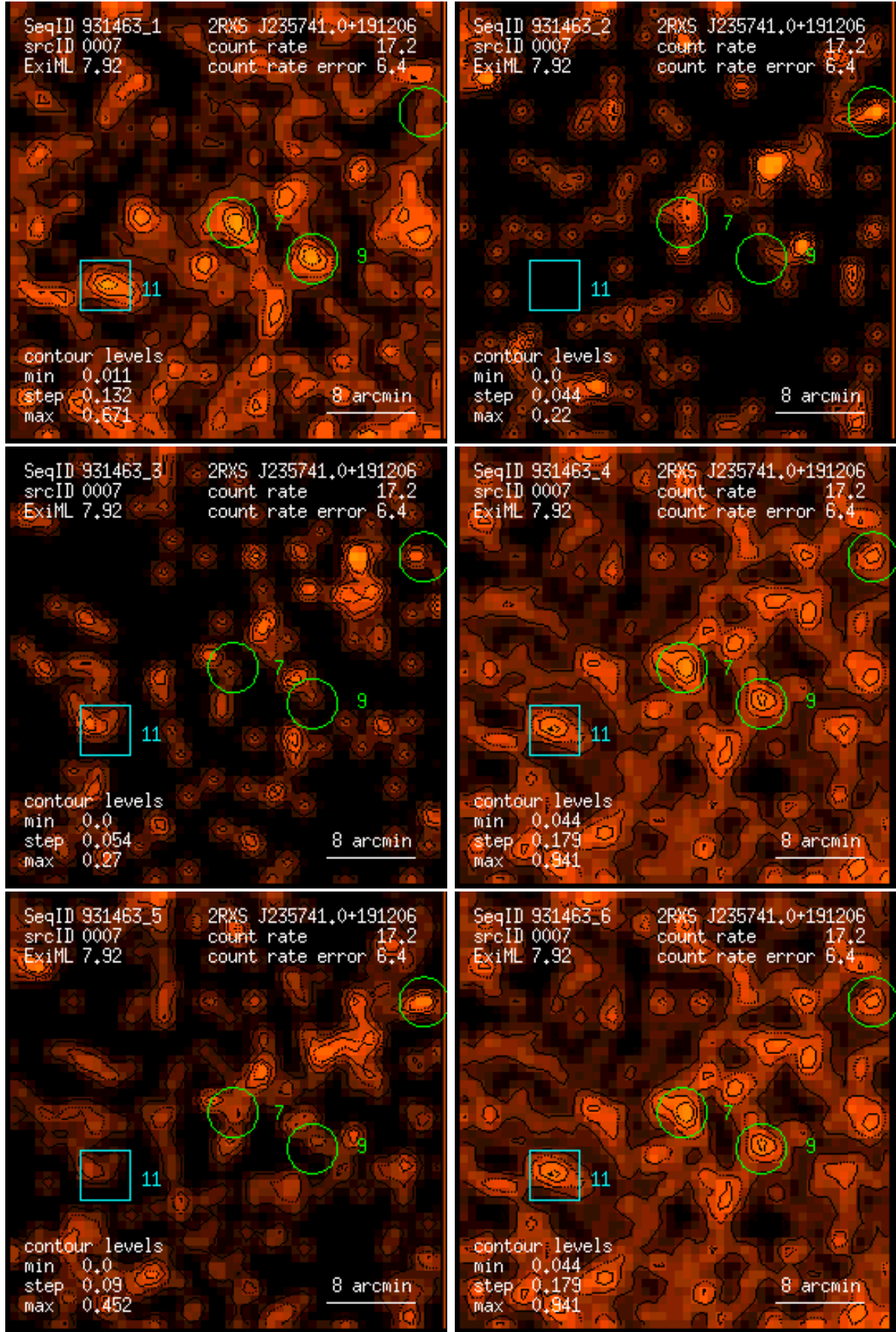
Figure 7: RASS 931463: detection 0007: band rate images, Gaussian filter: (1) PSPC channels 11 – 41, (2) 52 – 90, (3) 91 – 201, (4) 11 – 235, (5) 52 – 201, (6) 11 – 201. Broad band rates in counts/ks. Band rate contour levels in counts/ks/arcmin 2 .
