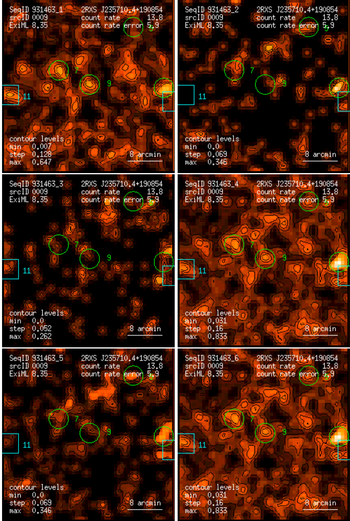
Figure 9: RASS 931463: detection 0009: band rate images, Gaussian filter: (1) PSPC channels 11 – 41, (2) 52 – 90, (3) 91 – 201, (4) 11 – 235, (5) 52 – 201, (6) 11 – 201. Broad band rates in counts/ks. Band rate contour levels in counts/ks/arcmin 2 .
