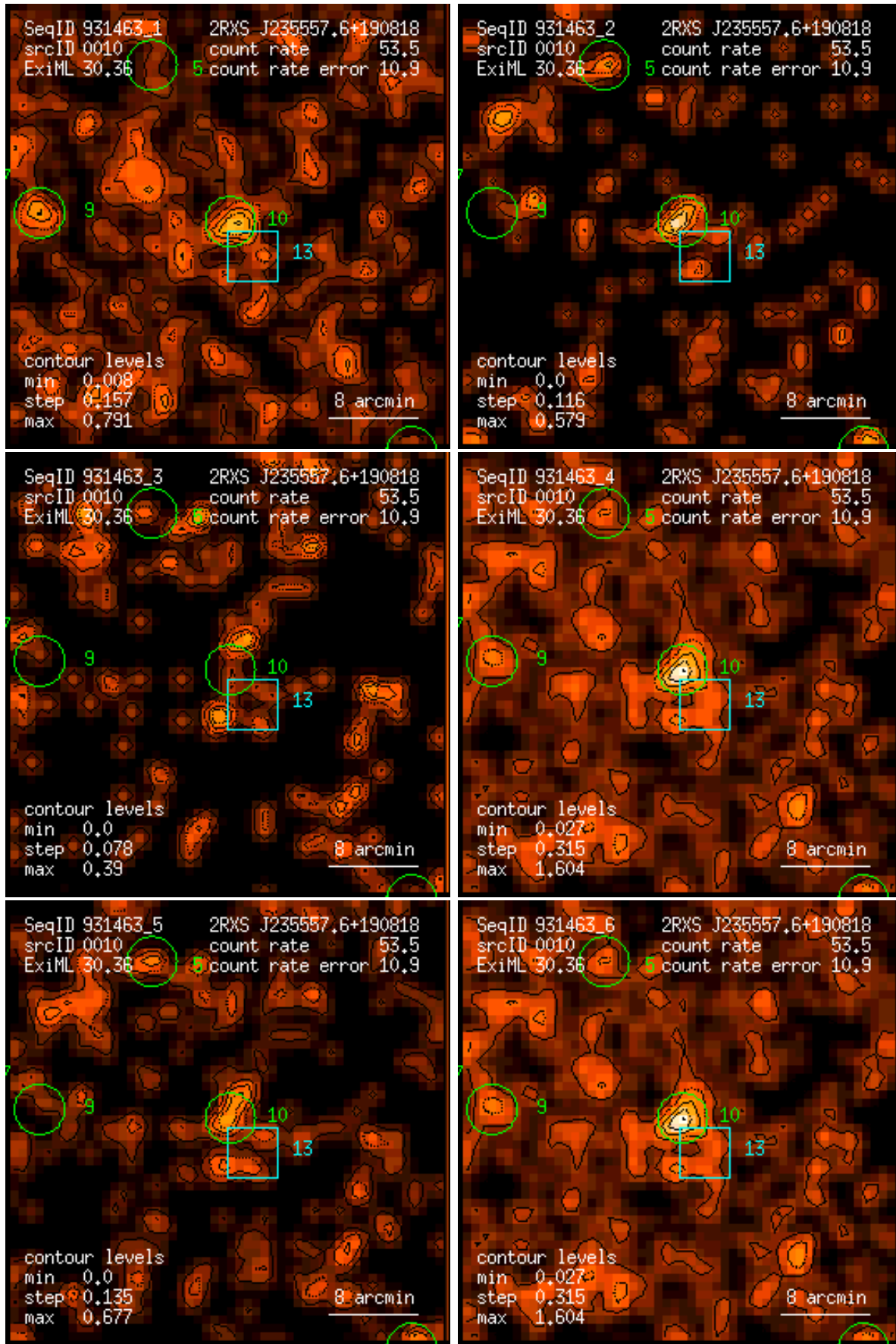
Figure 10: RASS 931463: detection 0010: band rate images, Gaussian filter: (1) PSPC channels 11 – 41, (2) 52 – 90, (3) 91 – 201, (4) 11 – 235, (5) 52 – 201, (6) 11 – 201. Broad band rates in counts/ks. Band rate contour levels in counts/ks/arcmin 2 .
