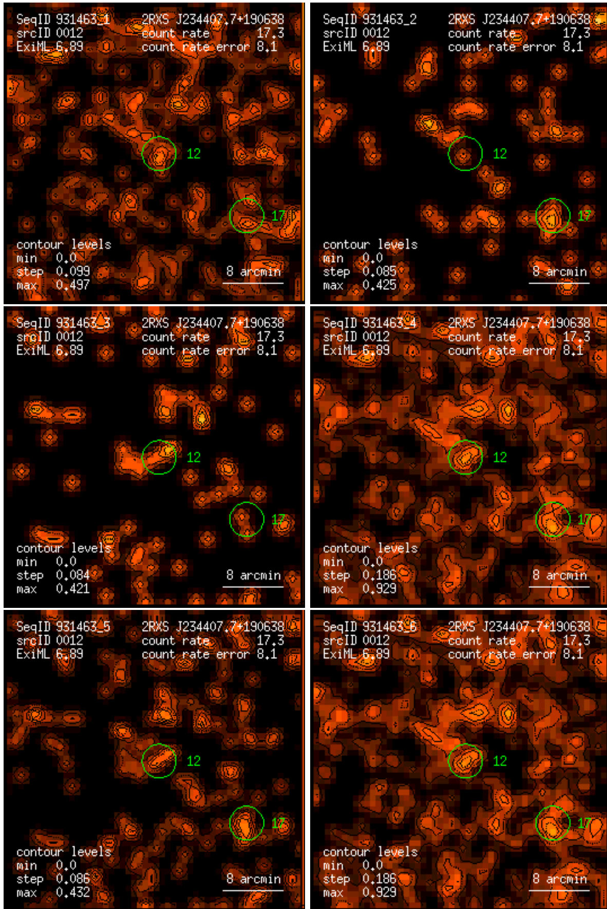
Figure 12: RASS 931463: detection 0012: band rate images, Gaussian filter: (1) PSPC channels 11 – 41, (2) 52 – 90, (3) 91 – 201, (4) 11 – 235, (5) 52 – 201, (6) 11 – 201. Broad band rates in counts/ks. Band rate contour levels in counts/ks/arcmin 2 .
