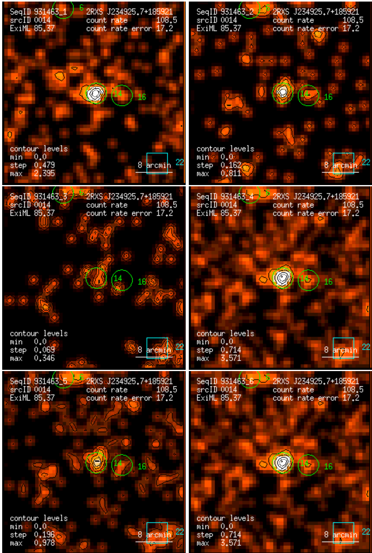
Figure 14: RASS 931463: detection 0014: band rate images, Gaussian filter: (1) PSPC channels 11 – 41, (2) 52 – 90, (3) 91 – 201, (4) 11 – 235, (5) 52 – 201, (6) 11 – 201. Broad band rates in counts/ks. Band rate contour levels in counts/ks/arcmin 2 .
