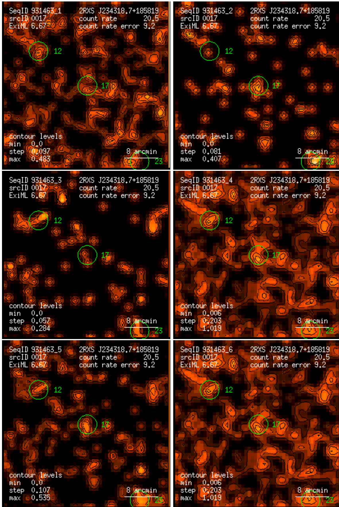
Figure 17: RASS 931463: detection 0017: band rate images, Gaussian filter: (1) PSPC channels 11 – 41, (2) 52 – 90, (3) 91 – 201, (4) 11 – 235, (5) 52 – 201, (6) 11 – 201. Broad band rates in counts/ks. Band rate contour levels in counts/ks/arcmin 2 .
