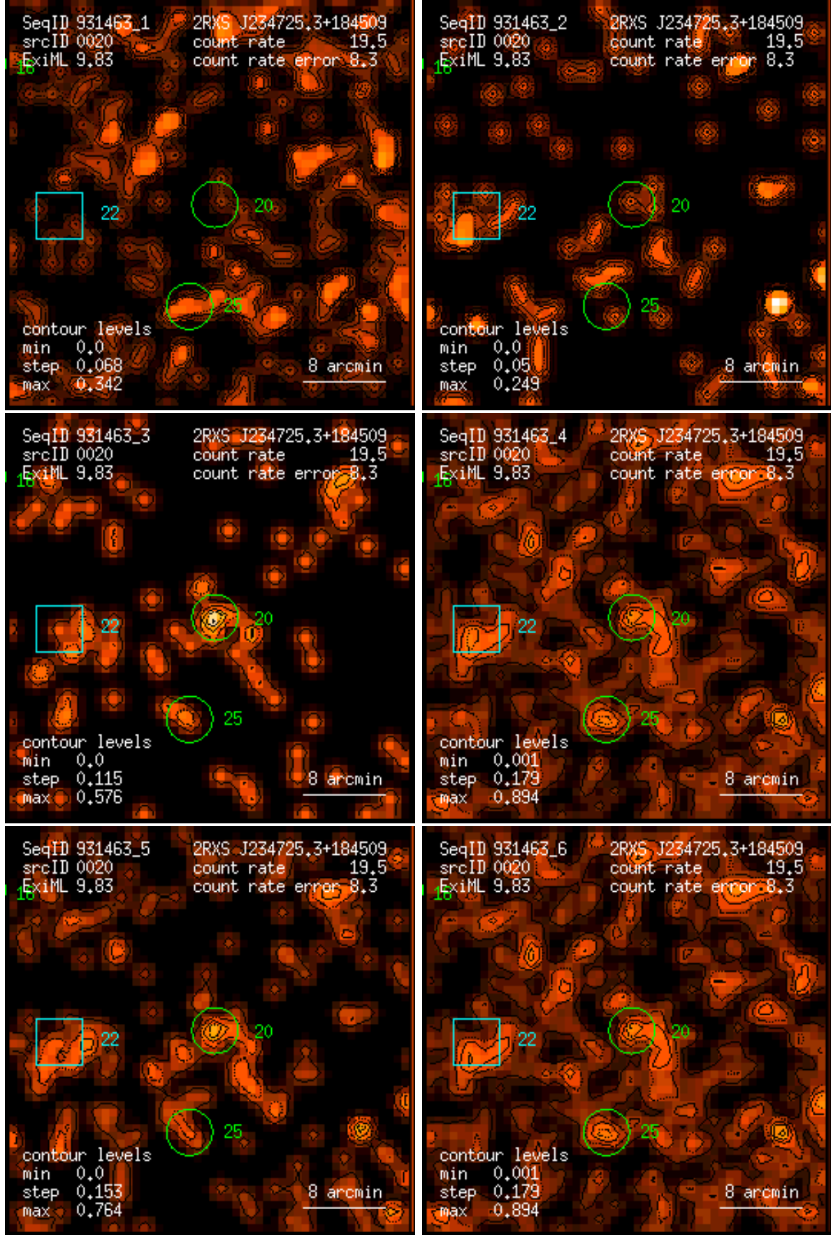
Figure 20: RASS 931463: detection 0020: band rate images, Gaussian filter: (1) PSPC channels 11 – 41, (2) 52 – 90, (3) 91 – 201, (4) 11 – 235, (5) 52 – 201, (6) 11 – 201. Broad band rates in counts/ks. Band rate contour levels in counts/ks/arcmin 2 .
