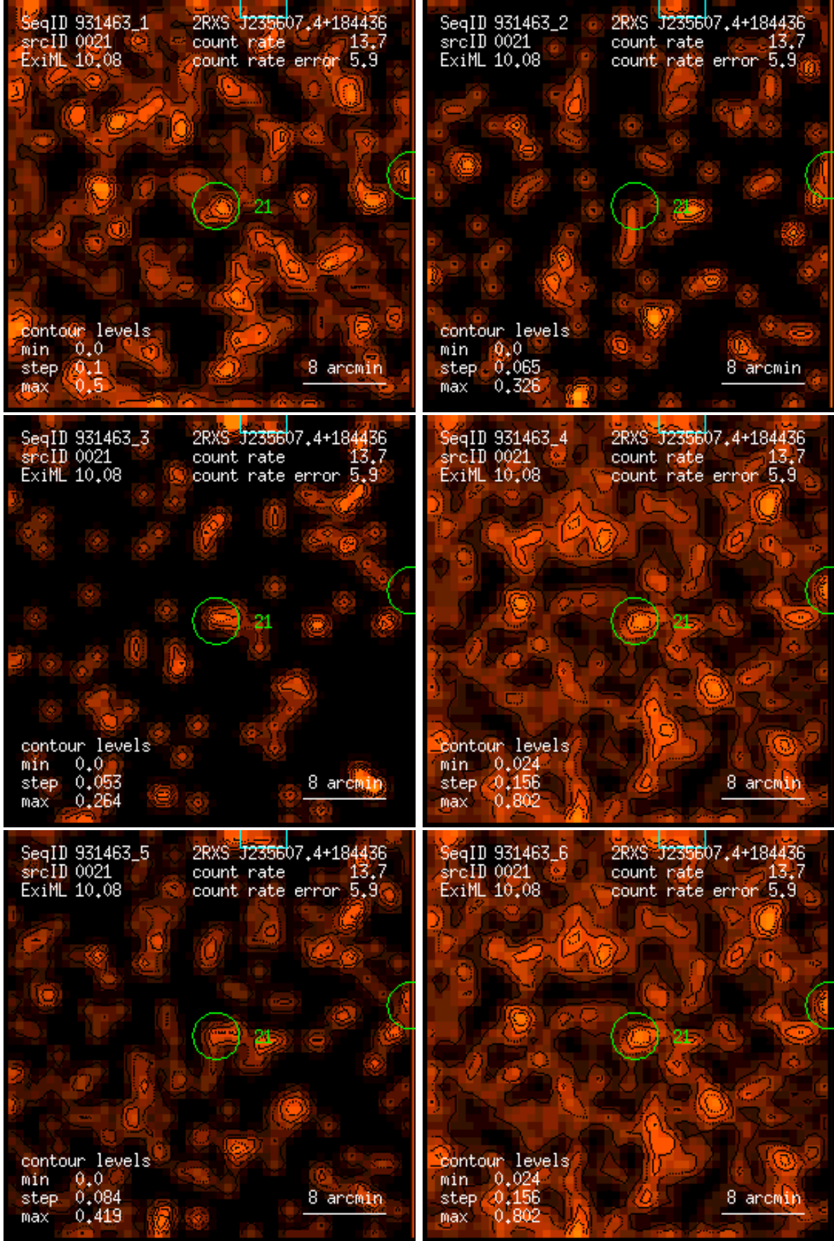
Figure 21: RASS 931463: detection 0021: band rate images, Gaussian filter: (1) PSPC channels 11 – 41, (2) 52 – 90, (3) 91 – 201, (4) 11 – 235, (5) 52 – 201, (6) 11 – 201. Broad band rates in counts/ks. Band rate contour levels in counts/ks/arcmin 2 .
