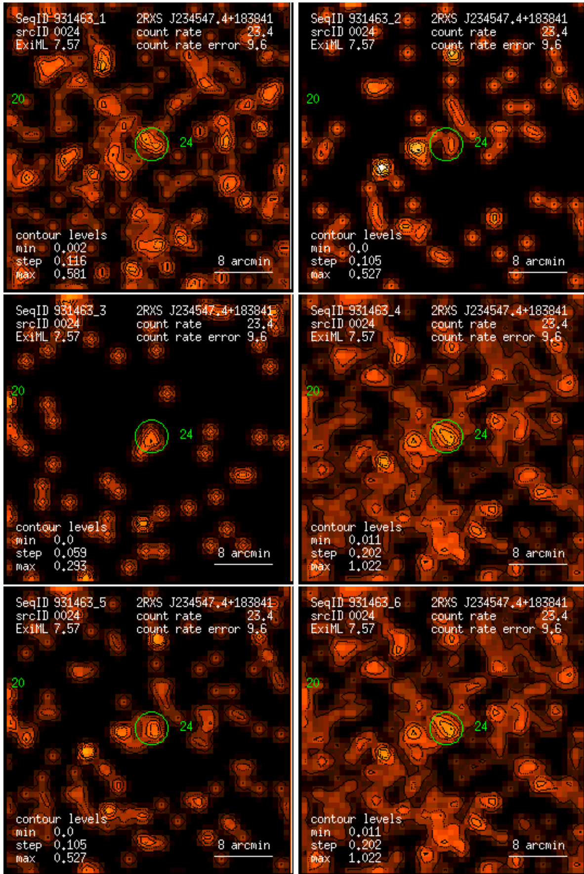
Figure 24: RASS 931463: detection 0024: band rate images, Gaussian filter: (1) PSPC channels 11 – 41, (2) 52 – 90, (3) 91 – 201, (4) 11 – 235, (5) 52 – 201, (6) 11 – 201. Broad band rates in counts/ks. Band rate contour levels in counts/ks/arcmin 2 .
