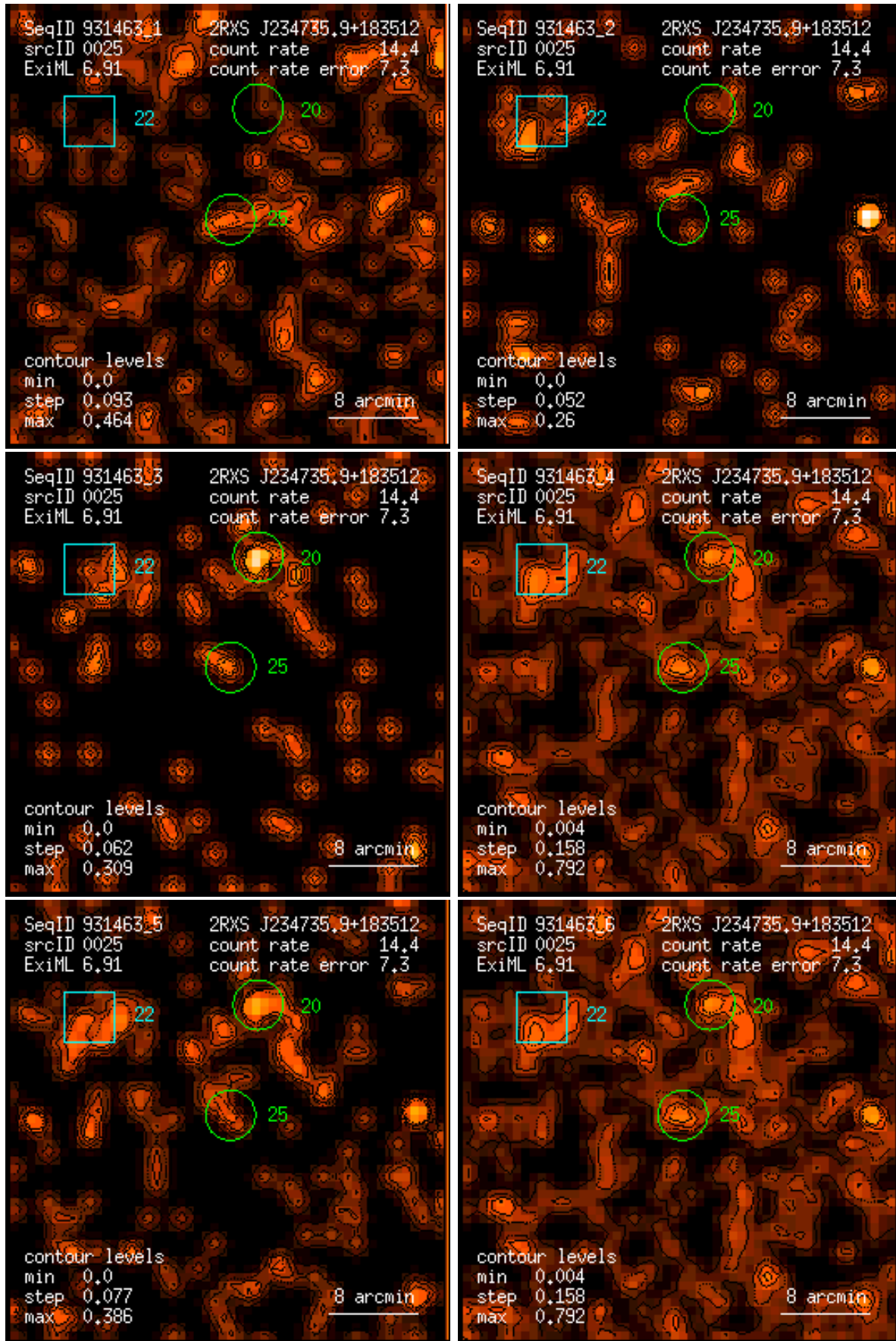
Figure 25: RASS 931463: detection 0025: band rate images, Gaussian filter: (1) PSPC channels 11 – 41, (2) 52 – 90, (3) 91 – 201, (4) 11 – 235, (5) 52 – 201, (6) 11 – 201. Broad band rates in counts/ks. Band rate contour levels in counts/ks/arcmin 2 .
