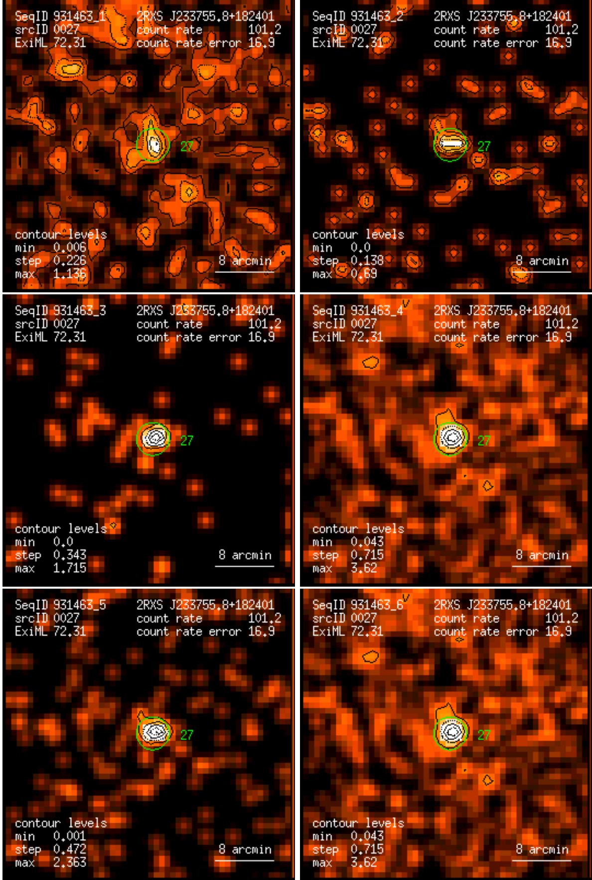
Figure 27: RASS 931463: detection 0027: band rate images, Gaussian filter: (1) PSPC channels 11 – 41, (2) 52 – 90, (3) 91 – 201, (4) 11 – 235, (5) 52 – 201, (6) 11 – 201. Broad band rates in counts/ks. Band rate contour levels in counts/ks/arcmin 2 .
