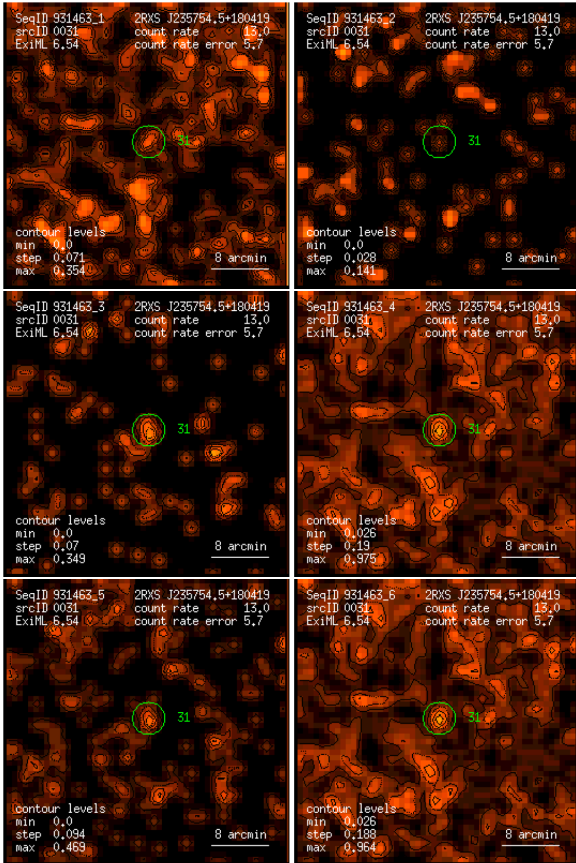
Figure 31: RASS 931463: detection 0031: band rate images, Gaussian filter: (1) PSPC channels 11 – 41, (2) 52 – 90, (3) 91 – 201, (4) 11 – 235, (5) 52 – 201, (6) 11 – 201. Broad band rates in counts/ks. Band rate contour levels in counts/ks/arcmin 2 .
