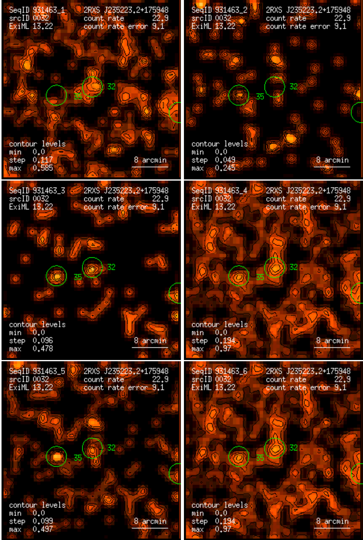
Figure 32: RASS 931463: detection 0032: band rate images, Gaussian filter: (1) PSPC channels 11 – 41, (2) 52 – 90, (3) 91 – 201, (4) 11 – 235, (5) 52 – 201, (6) 11 – 201. Broad band rates in counts/ks. Band rate contour levels in counts/ks/arcmin 2 .
