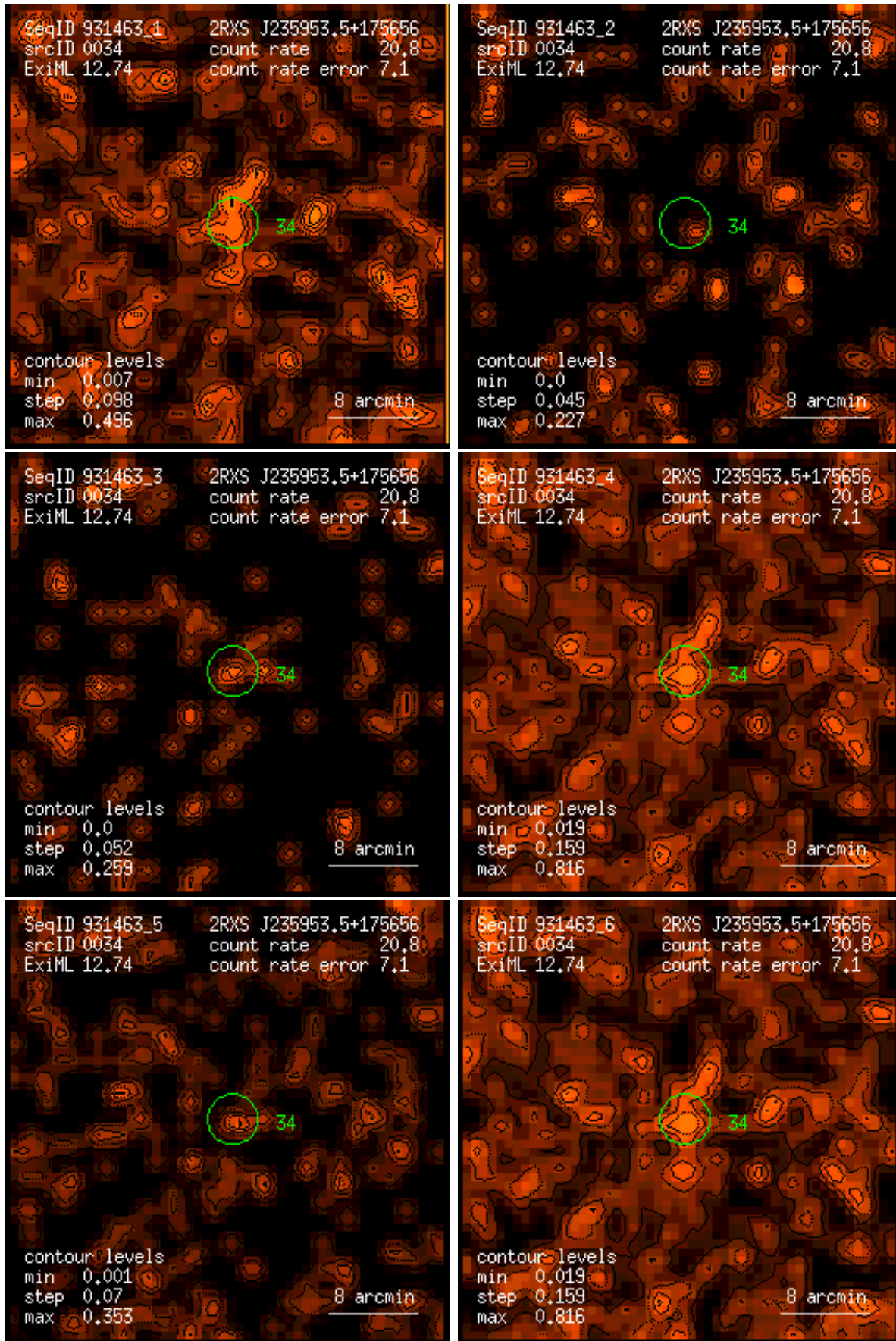
Figure 34: RASS 931463: detection 0034: band rate images, Gaussian filter: (1) PSPC channels 11 – 41, (2) 52 – 90, (3) 91 – 201, (4) 11 – 235, (5) 52 – 201, (6) 11 – 201. Broad band rates in counts/ks. Band rate contour levels in counts/ks/arcmin 2 .
