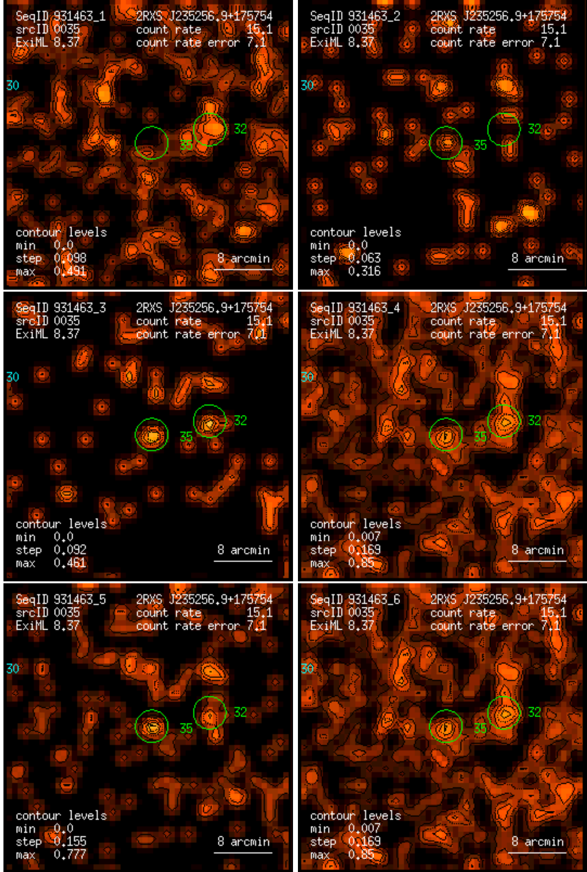
Figure 35: RASS 931463: detection 0035: band rate images, Gaussian filter: (1) PSPC channels 11 – 41, (2) 52 – 90, (3) 91 – 201, (4) 11 – 235, (5) 52 – 201, (6) 11 – 201. Broad band rates in counts/ks. Band rate contour levels in counts/ks/arcmin 2 .
