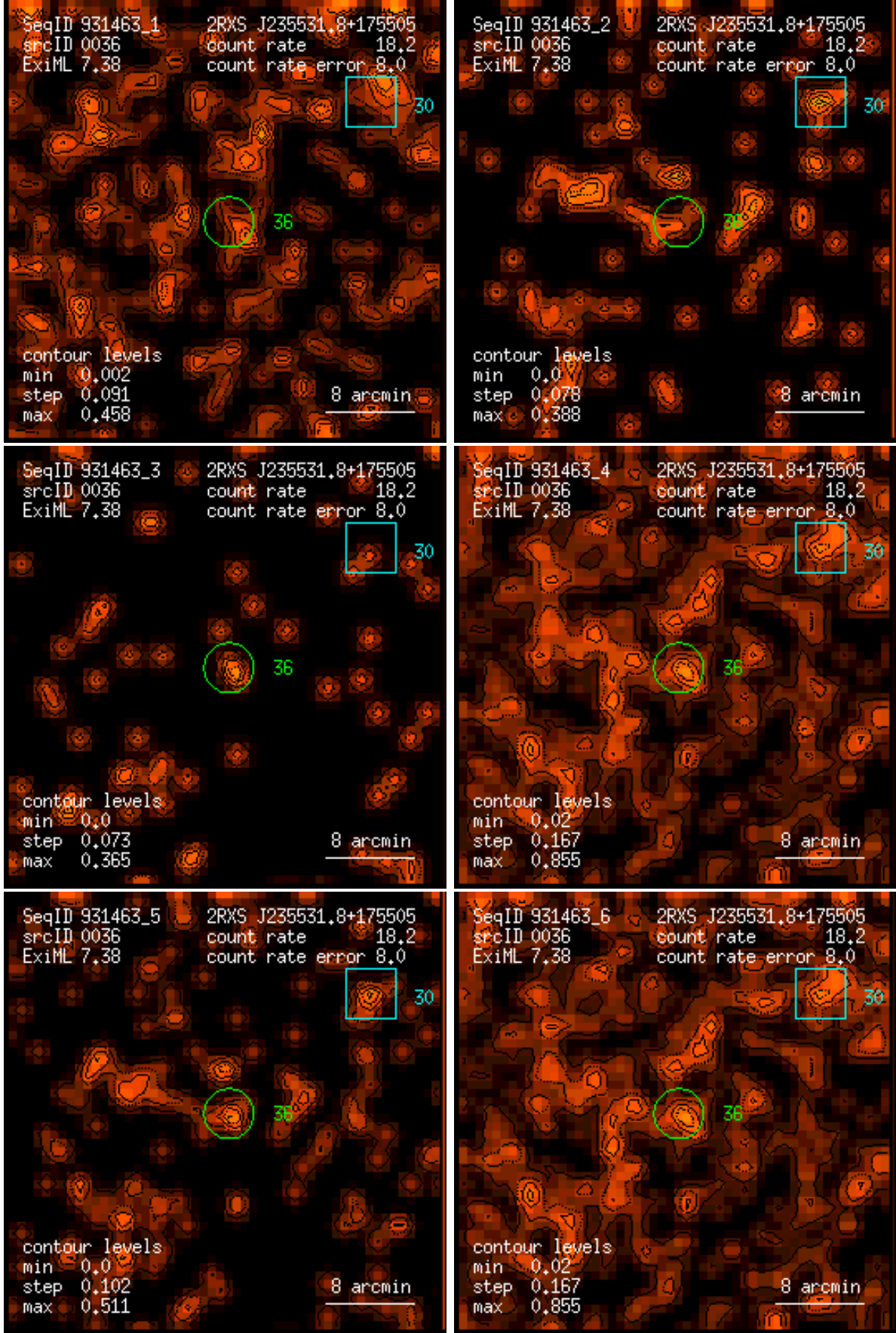
Figure 36: RASS 931463: detection 0036: band rate images, Gaussian filter: (1) PSPC channels 11 – 41, (2) 52 – 90, (3) 91 – 201, (4) 11 – 235, (5) 52 – 201, (6) 11 – 201. Broad band rates in counts/ks. Band rate contour levels in counts/ks/arcmin 2 .
