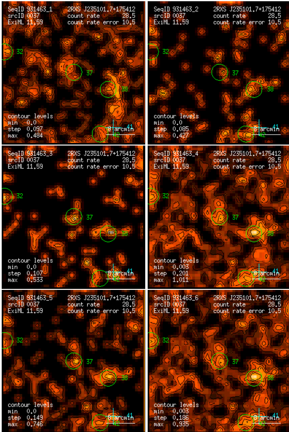
Figure 37: RASS 931463: detection 0037: band rate images, Gaussian filter: (1) PSPC channels 11 – 41, (2) 52 – 90, (3) 91 – 201, (4) 11 – 235, (5) 52 – 201, (6) 11 – 201. Broad band rates in counts/ks. Band rate contour levels in counts/ks/arcmin 2 .
