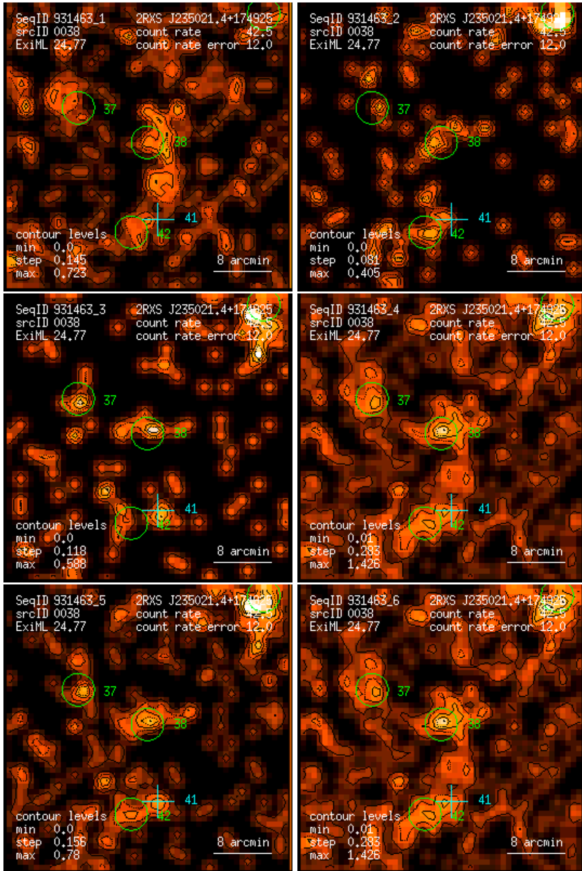
Figure 38: RASS 931463: detection 0038: band rate images, Gaussian filter: (1) PSPC channels 11 – 41, (2) 52 – 90, (3) 91 – 201, (4) 11 – 235, (5) 52 – 201, (6) 11 – 201. Broad band rates in counts/ks. Band rate contour levels in counts/ks/arcmin 2 .
