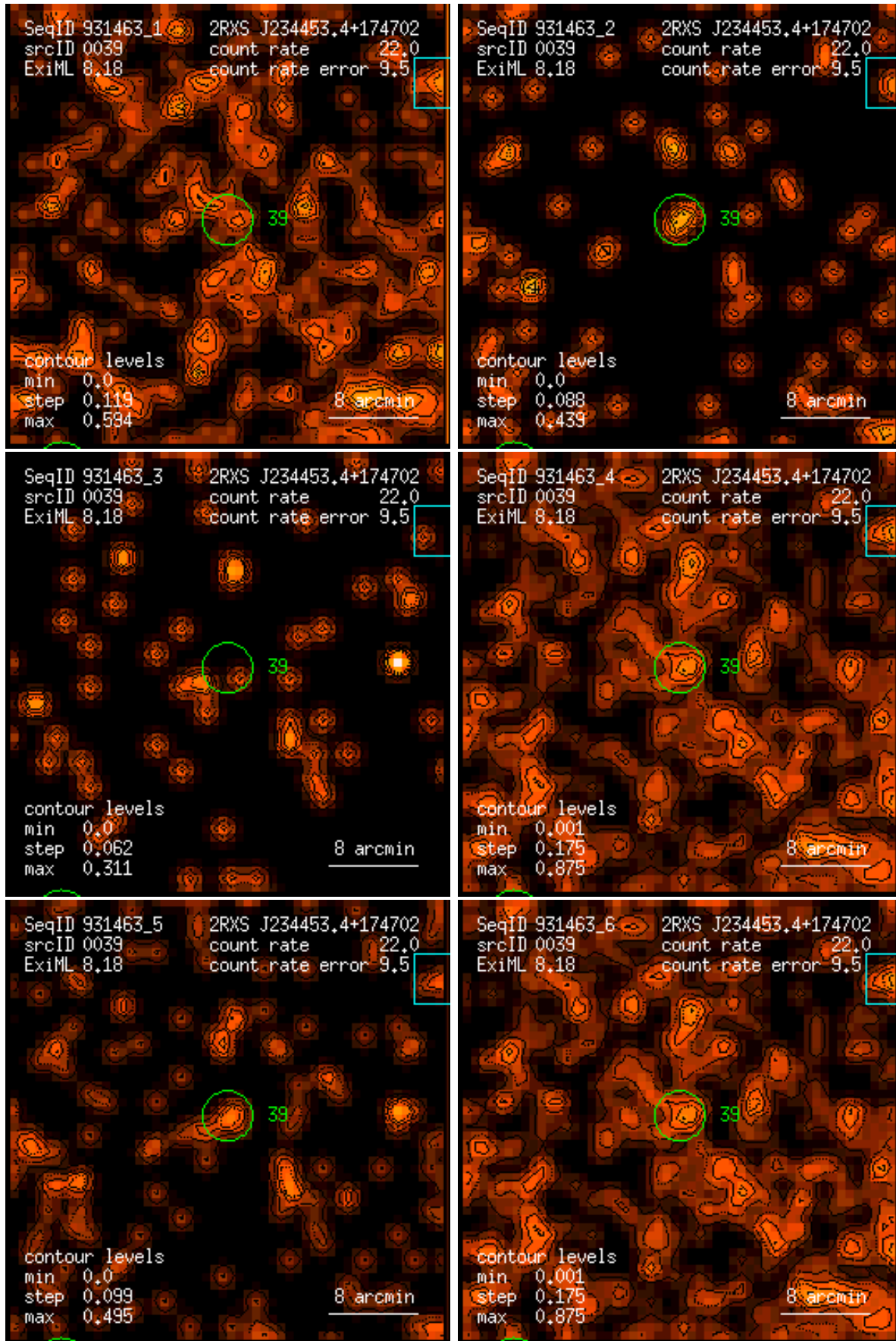
Figure 39: RASS 931463: detection 0039: band rate images, Gaussian filter: (1) PSPC channels 11 – 41, (2) 52 – 90, (3) 91 – 201, (4) 11 – 235, (5) 52 – 201, (6) 11 – 201. Broad band rates in counts/ks. Band rate contour levels in counts/ks/arcmin 2 .
